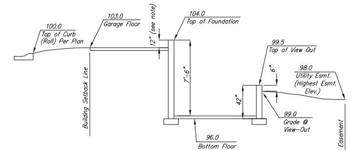
* Varies (Check Individual Lot) Section Through Typical View-Out Lot
