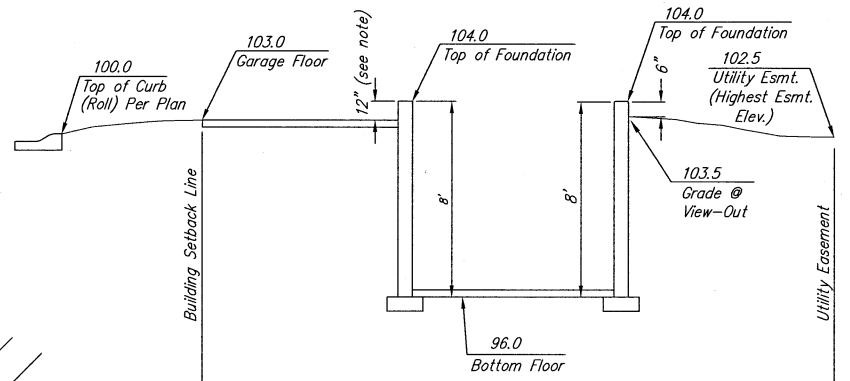
Section Through Typical Full Basement
