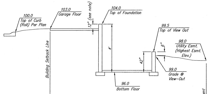
Section Through Typical View-Out Lot
