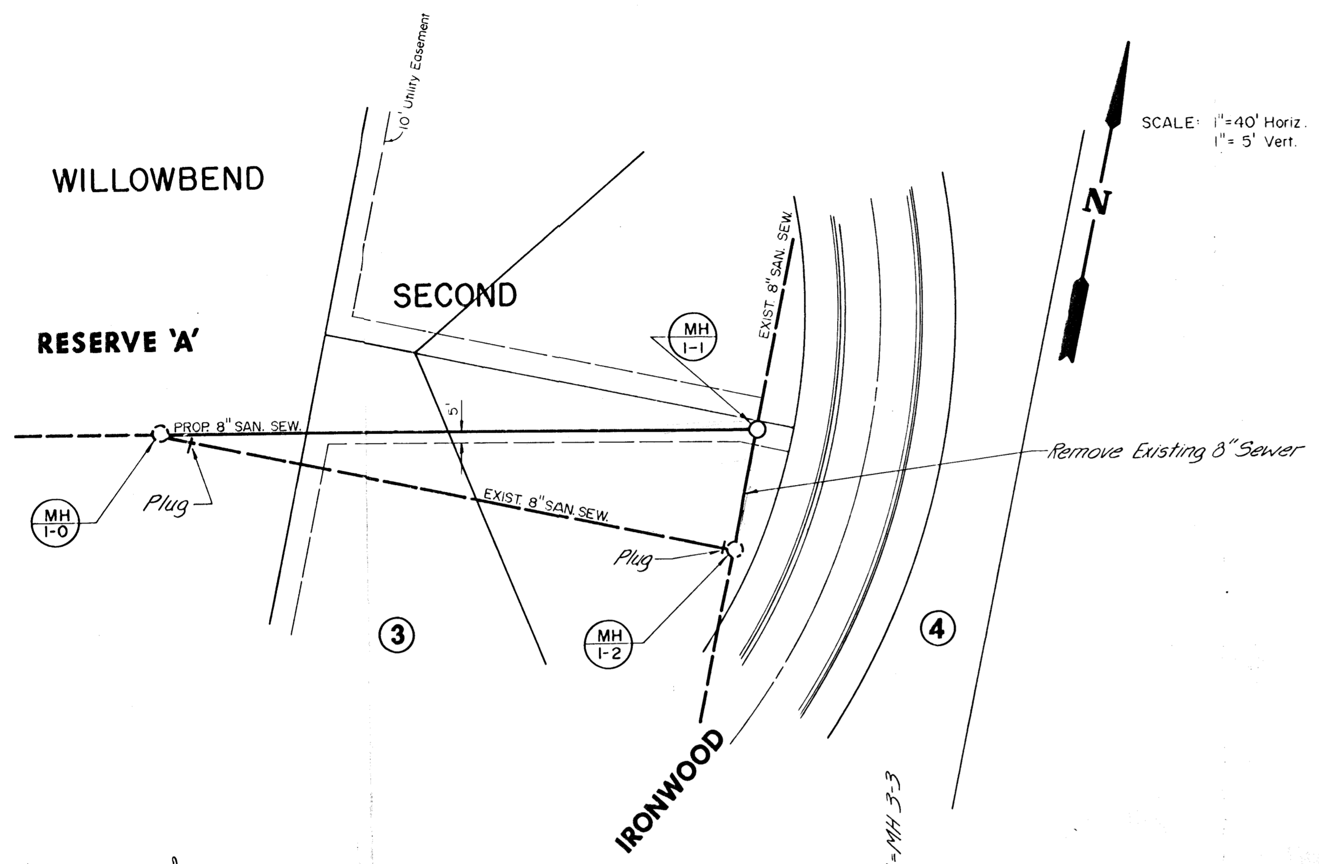
PLAN LINE I PROFILE LINE I
