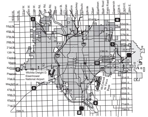
Vicinity Map
