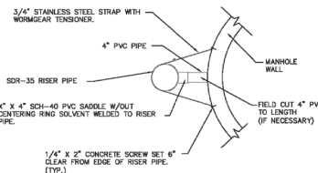
RISE PIPE RESTRAINING ASSEMBLY Not to Scale
