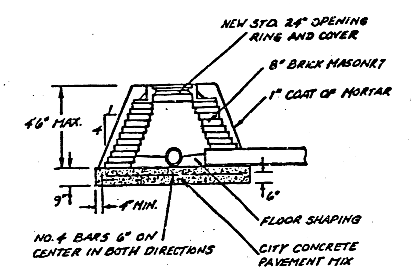
SPECIAL SHALLOW TYPE "A" MANHOLE
