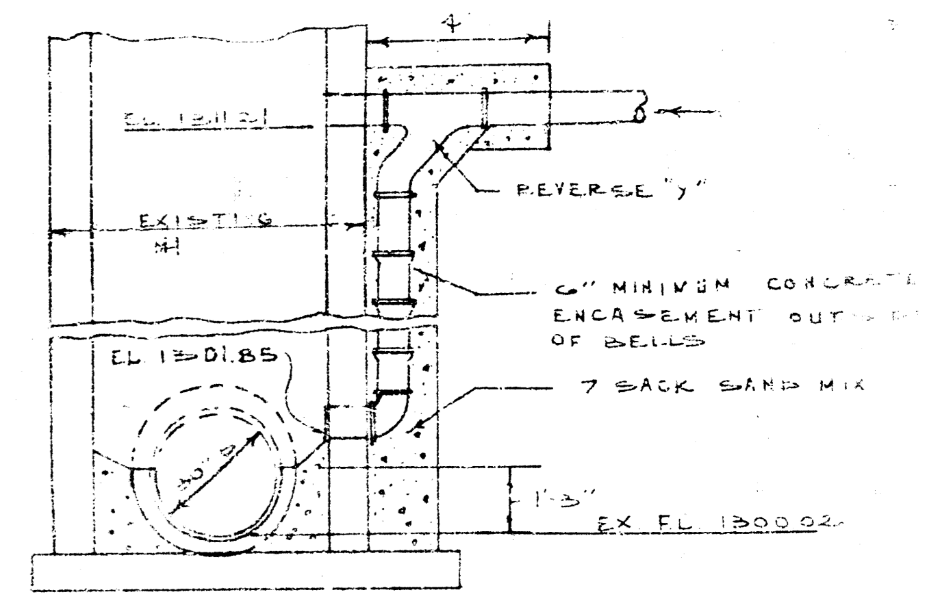
SECTION I OUTSIDE PROP INTO EXISTING M.D.100
