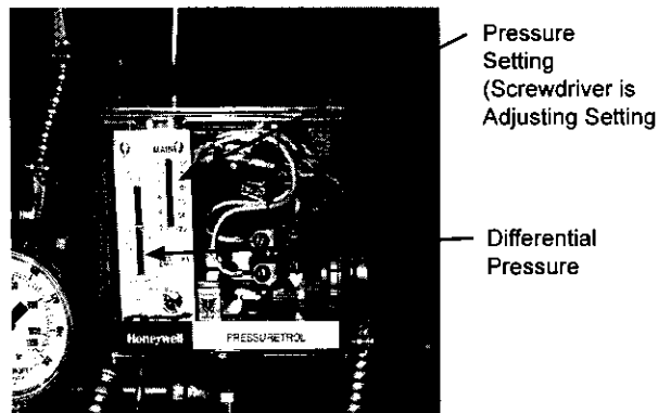
Figure E-10 Low Oil and Atomizing Air Pressure Switches
