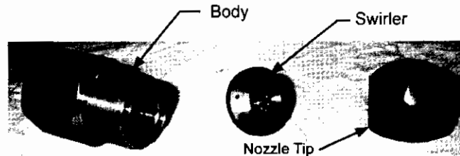
Figure B-14 Typical Small Air Atomizing Oil Nozzle
