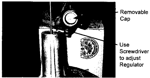
Figure E-7 Main Gas Pressure Regulator Adjustment
