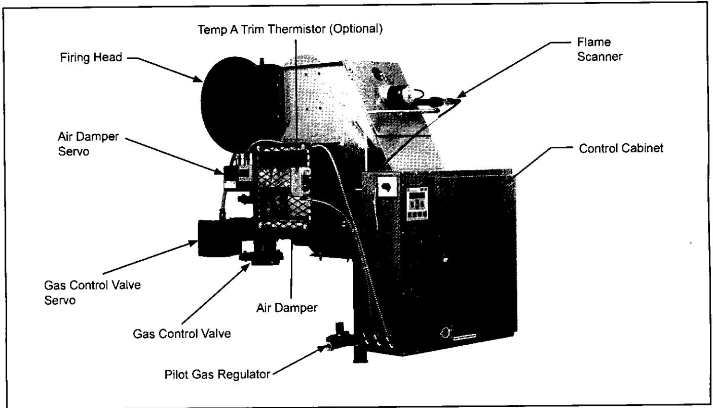
Figure B-1: JBS2G With Parallel Positioning Control, Temp A Trim And Rear Mounted Panel
