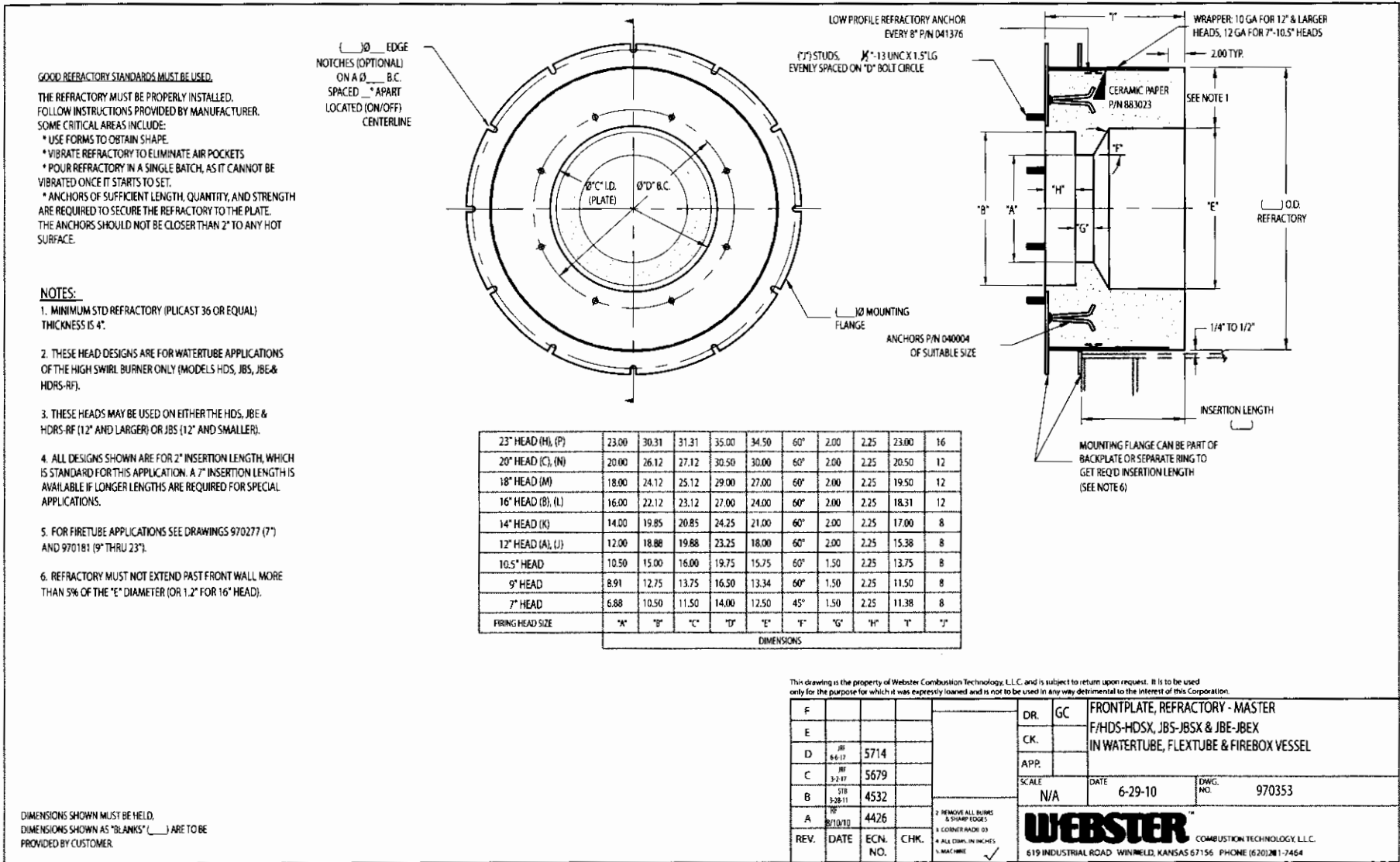
Figure C-3 Refractory Watertube Boilers
