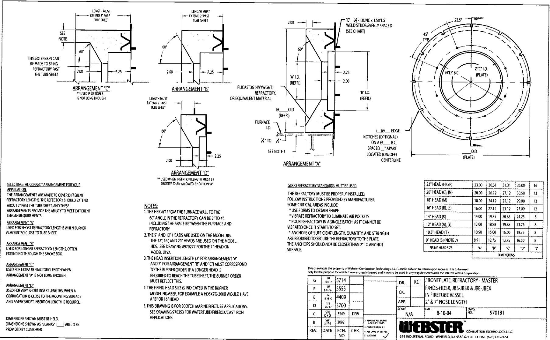
Figure C-2 Refractory Firetube Boilers
