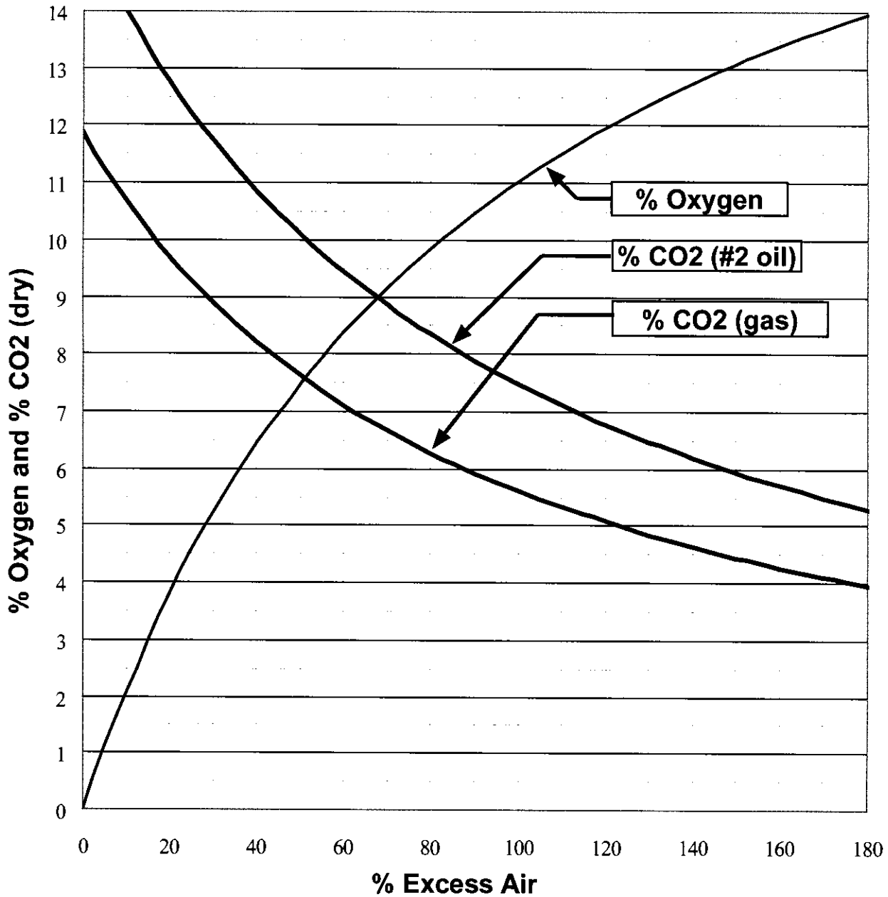
Excess Air vs. % Oxygen and % CO 2
