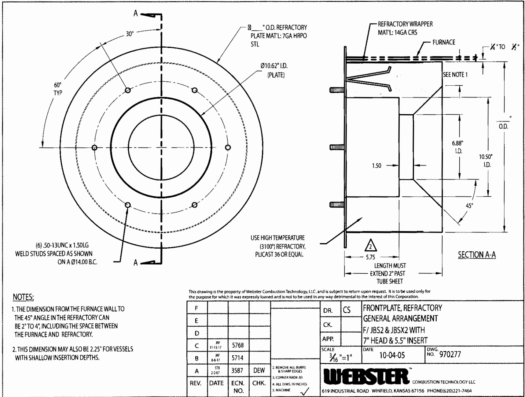
Figure C-1 Scotch-Type Refractory Boilers
