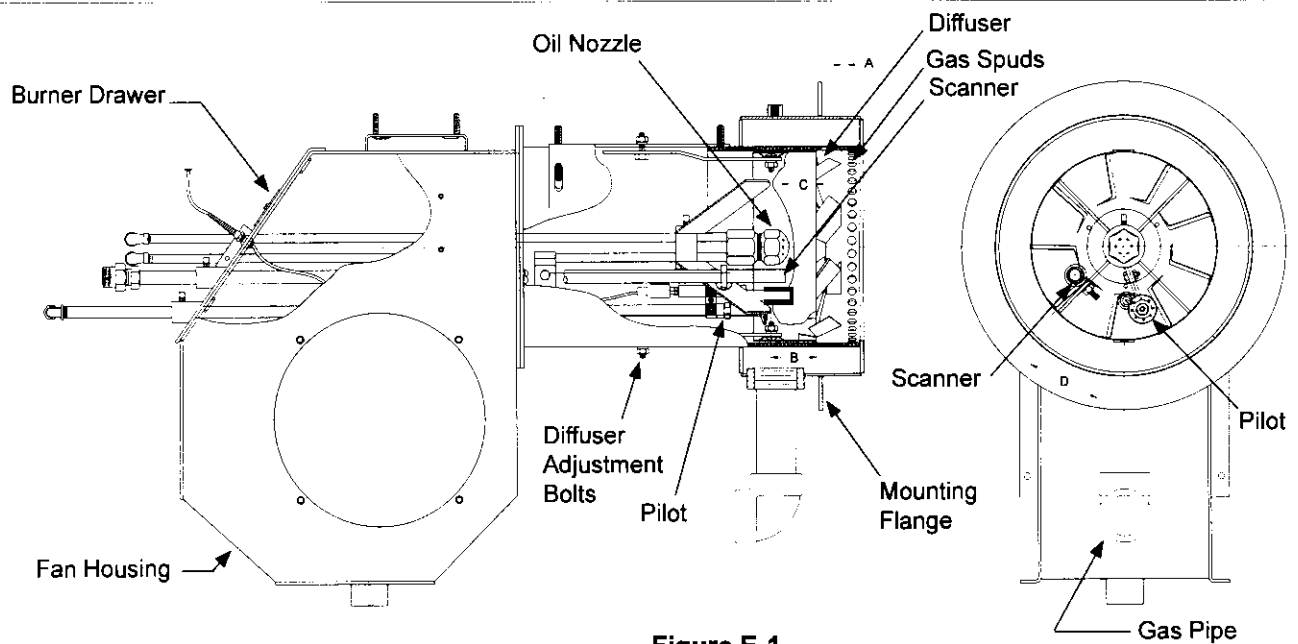
Figure E-1 Burner Drawer Setup
