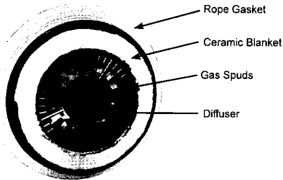
Figure C-10 Ceramic Blanket and Rope Gasket
