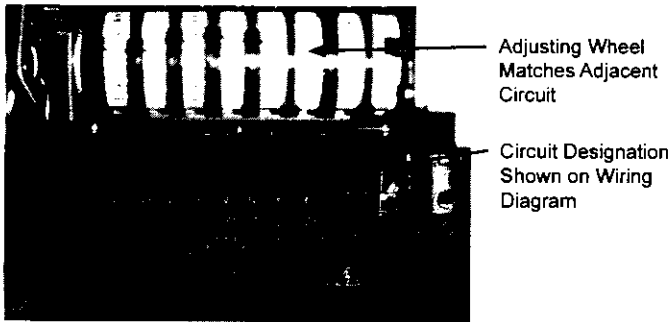
Figure E-3 Multiple Setpoint Modulation Motor (Siemens)
