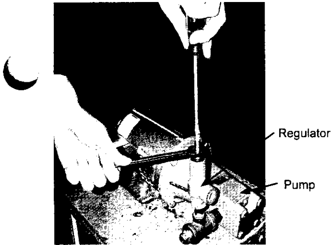
Figure E-9 Oil Pressure Regulator Adjustment
