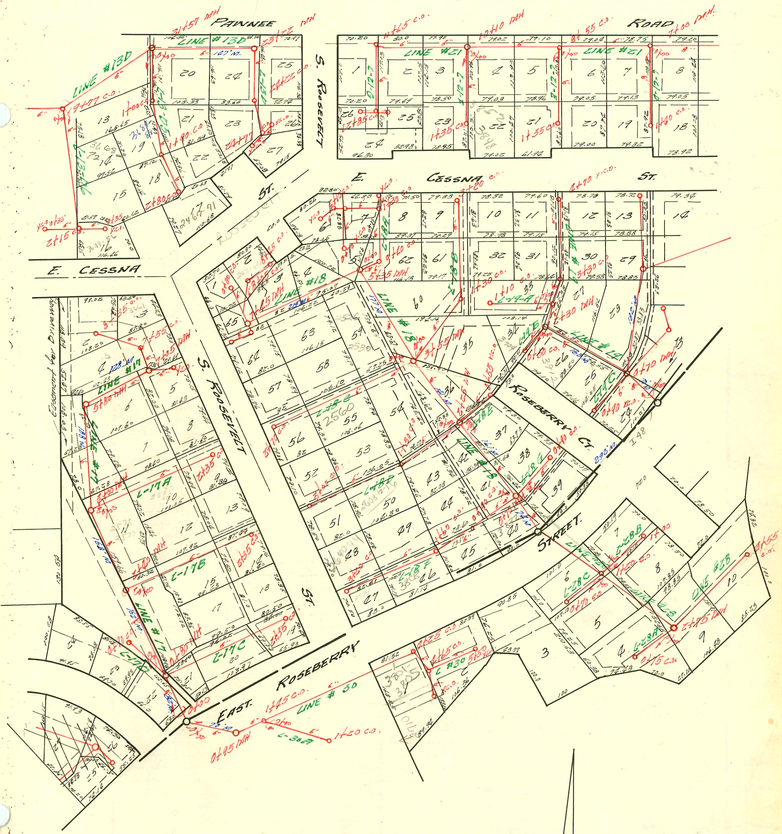
PLANEVIEW SANITARY SEWER NOTE: DO NOT SCALE FOR MEASUREMENT.
