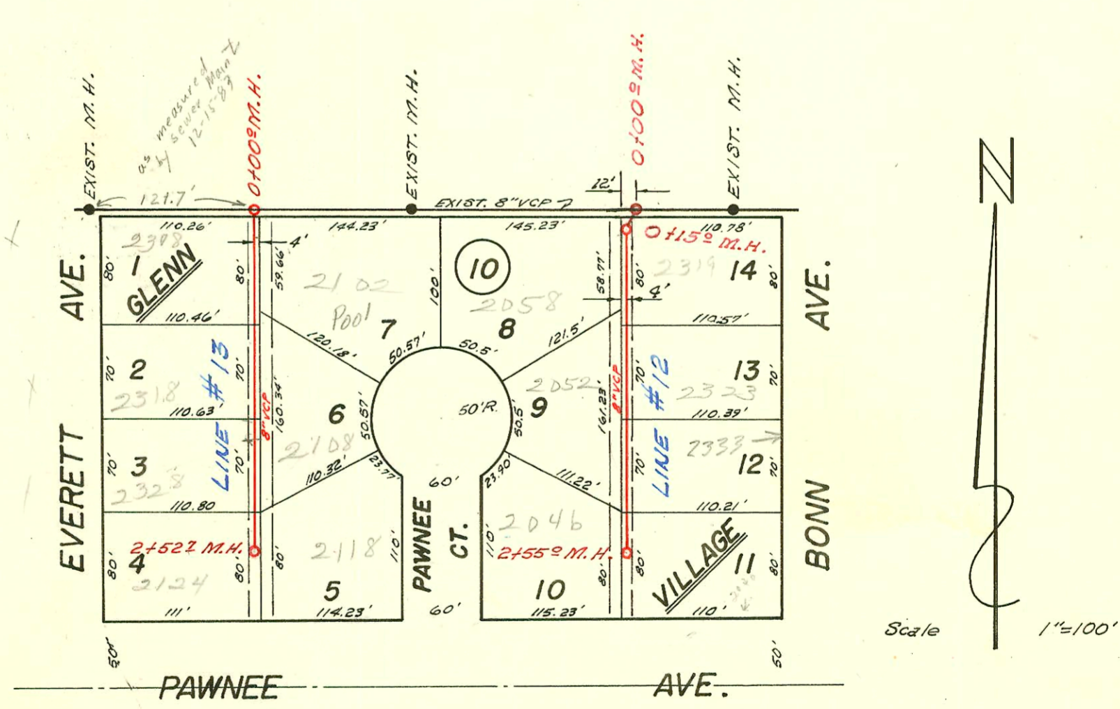
PART OF GLENN VILLAGE SANITARY SEWERS
