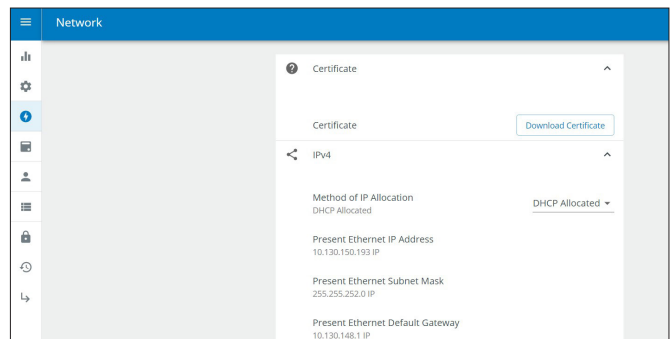
Figure 29. Download certificate
