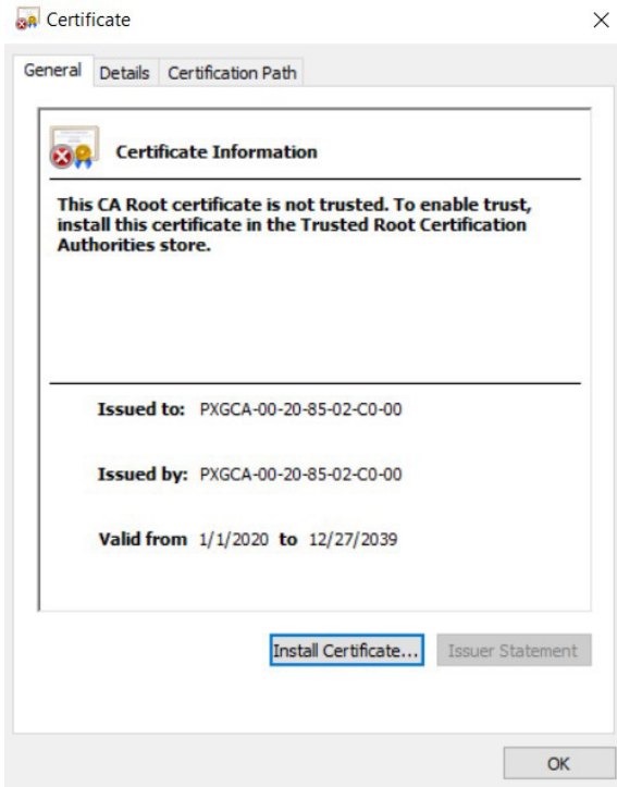
Figure 35. Install certificate
