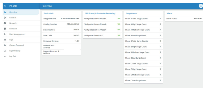
Figure 42. Log screen
