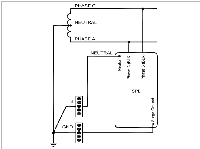
Figure 7. Wiring - split phase units
