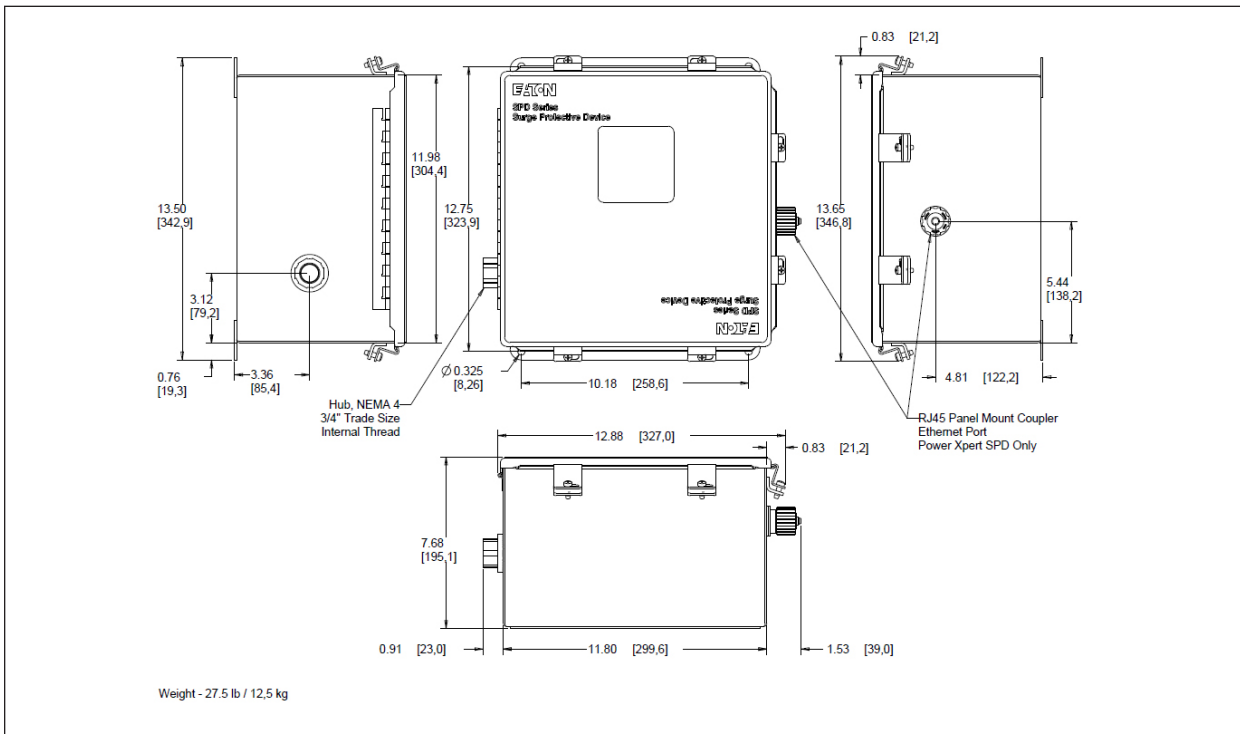
Figure 6. NEMA 4-4X (with disconnect) (suffix O, Q) (NEMA 4X not available with Power Xpert SPD)
