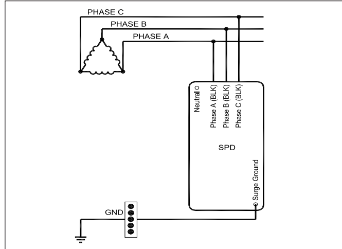
Figure 8. Wiring - 3-phase delta units
