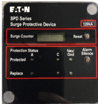
Figure 21. Standard with Surge Counter feature package display
