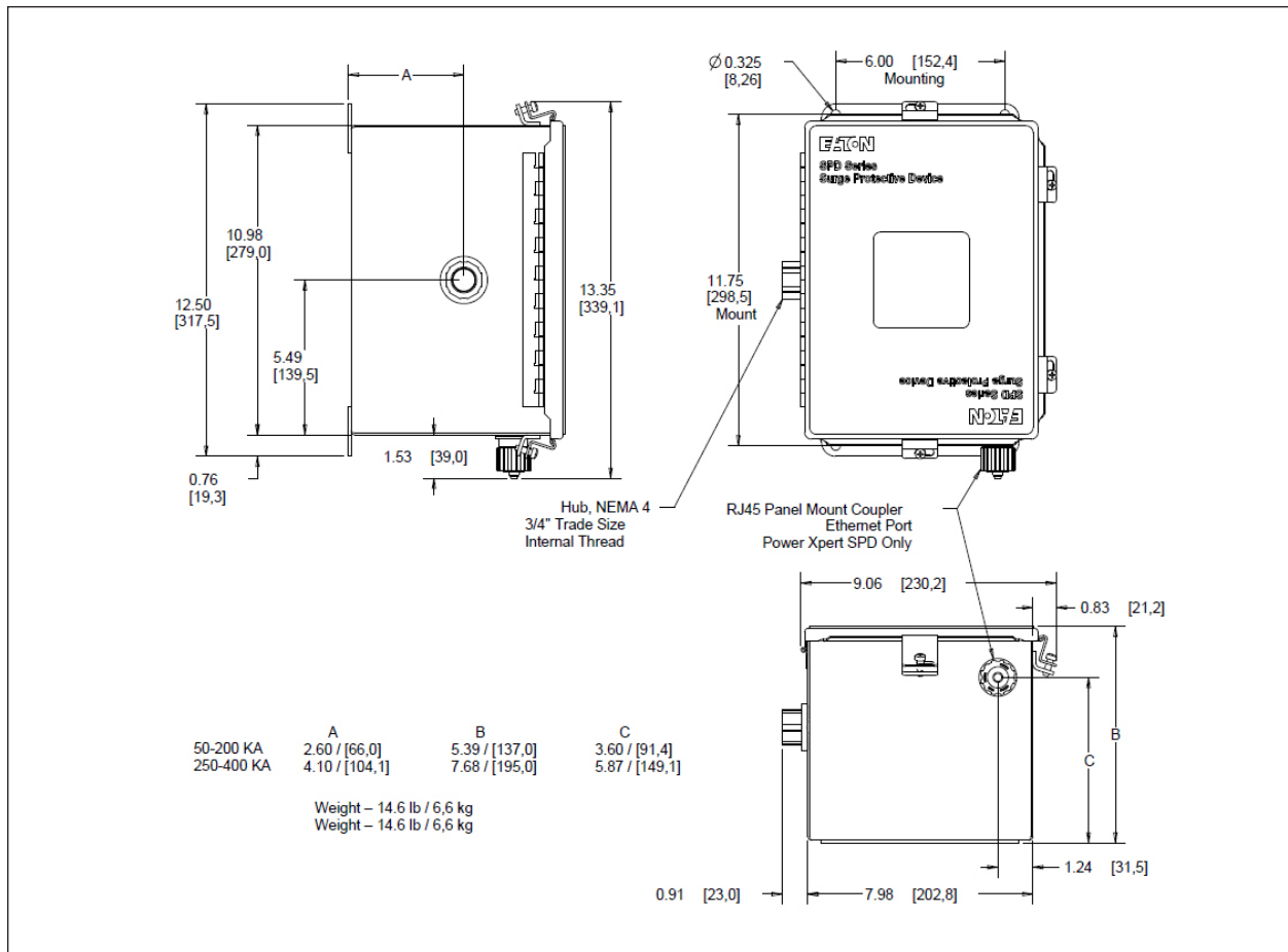
Figure 4. NEMA 4 - 4X (suffix N, P) (NEMA 4X not available with Power Xpert SPD)
