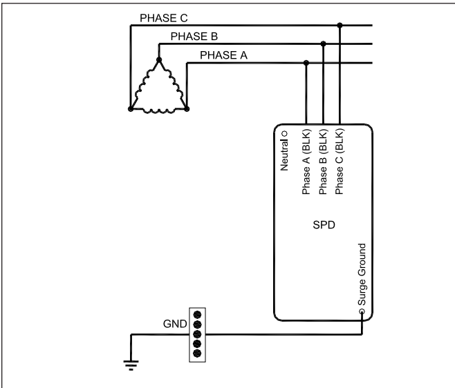
Figure 10. 3-phase delta
