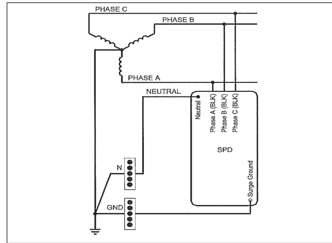
Figure 9. Wiring - 3-phase wye units
