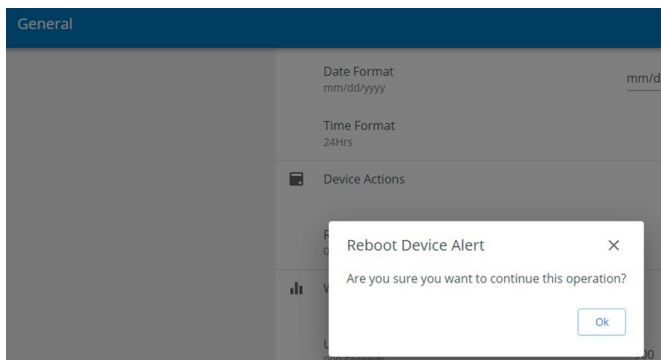
Figure 55. Confirm reboot
