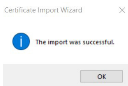
Figure 35. Import successful
