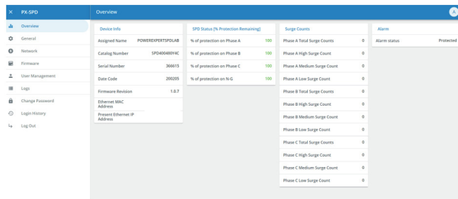
Figure 47. Log screen
