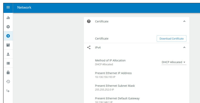
Figure 34. Download certificate
