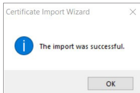
Figure 40. Import successful
