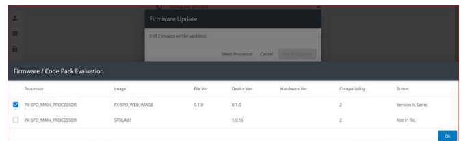
Figure 39. Select PX-SPD_Main_Processor
