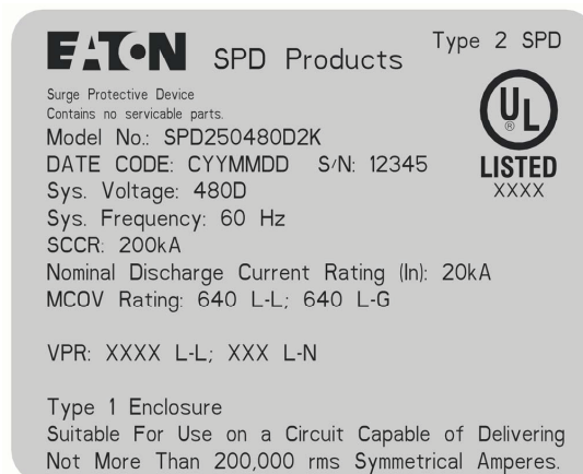
Figure 1. Product label
