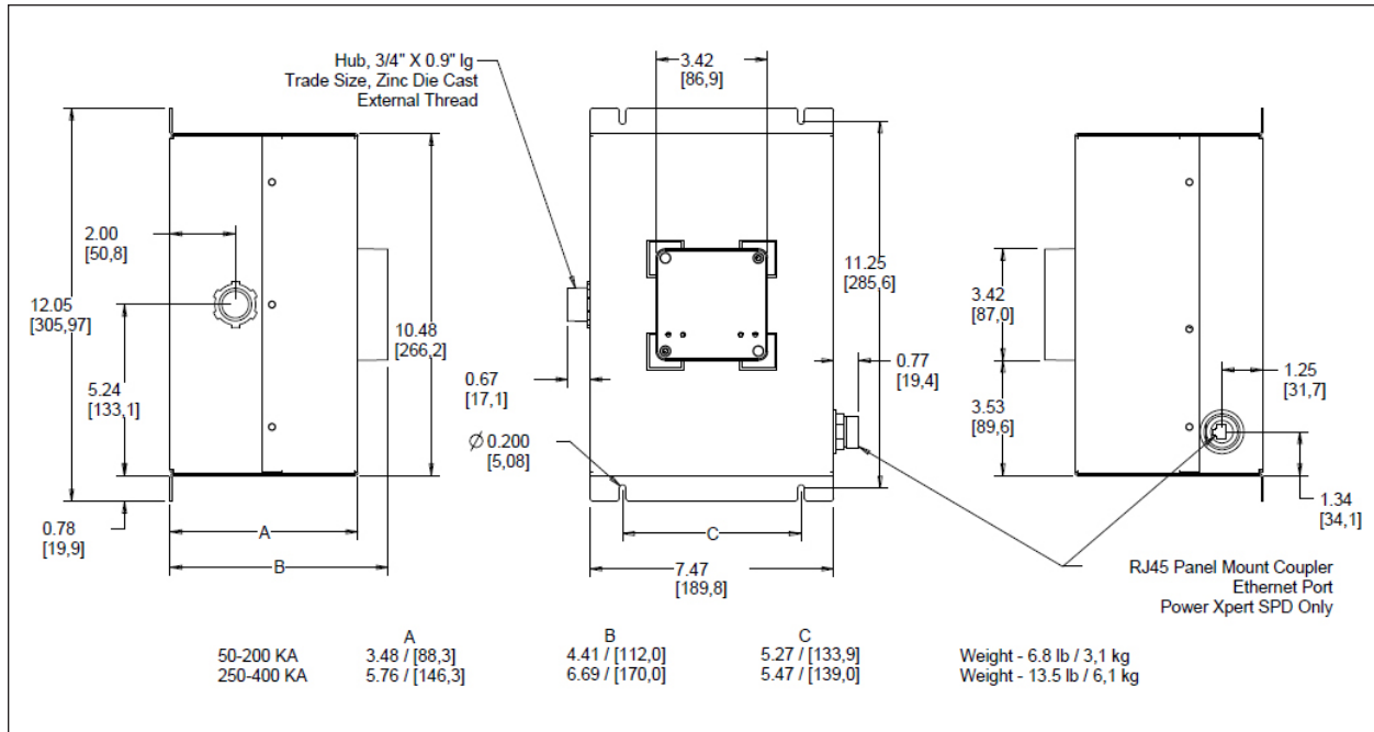
Figure 3. NEMA 1 (suffix K)
