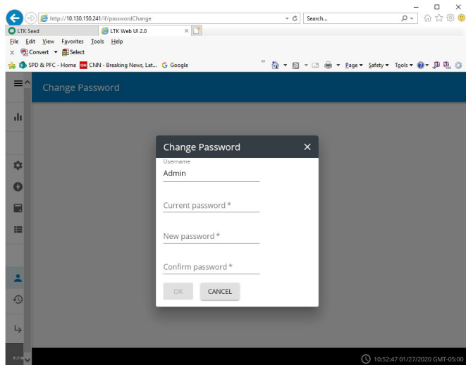
Figure 33. Password screen
