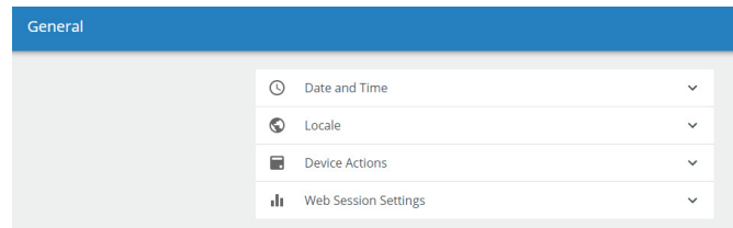
Figure 50. General settings
