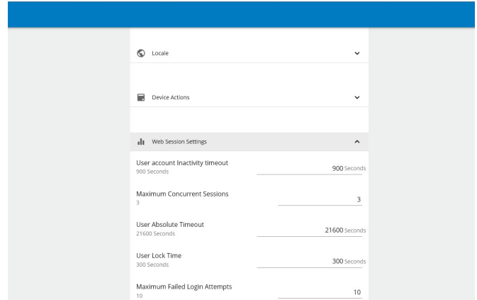
Figure 50. Modifying timeouts
