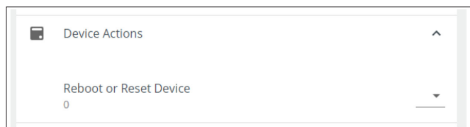
Figure 53. Device actions
