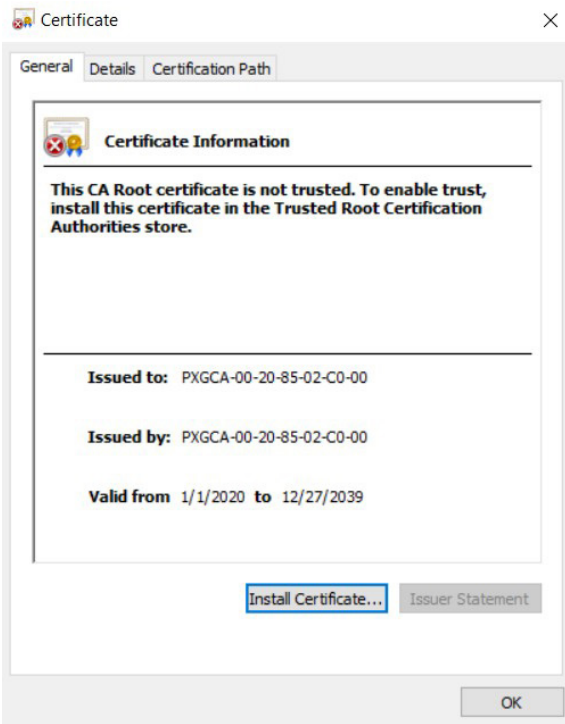
Figure 30. Install certificate
