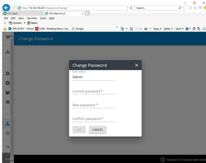
Figure 28. Password screen
