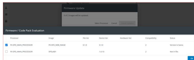
Figure 44. Select PX-SPD_Main_Processor
