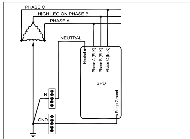
Figure 10. Wiring - high leg delta units
