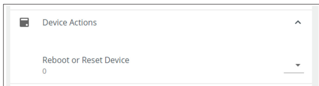
Figure 48. Device actions
