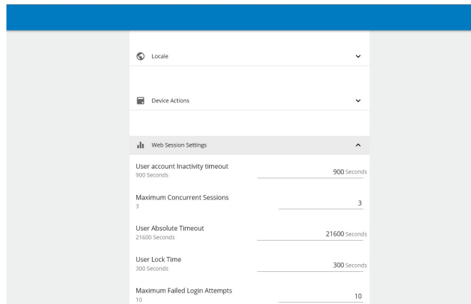
Figure 55. Modifying timeouts
