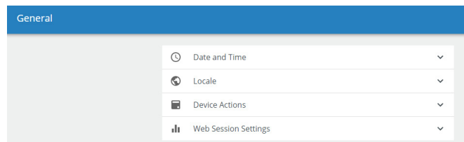
Figure 45. General settings
