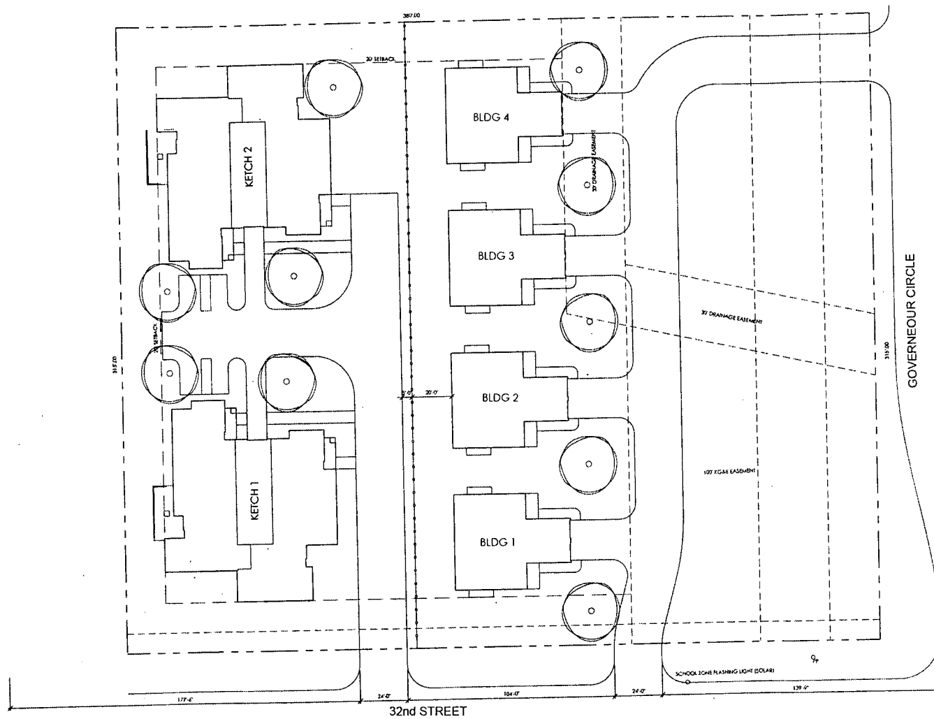
A SITE DEVELOPMENT PLAN 1"=20'-0"
