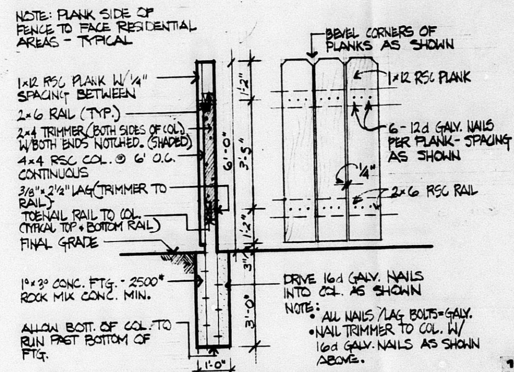
TYPICAL FENCE DETAIL SCALE: 1/2" = 1'-0"
