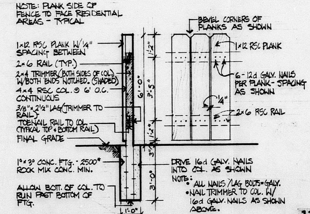
TYPICAL FENCE DETAIL SCALE: 1/2" = 1'-0"
