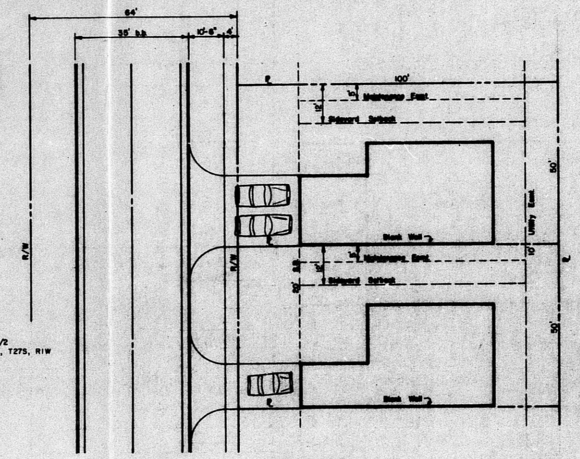
TYPICAL SCALE: 1" = 20'
