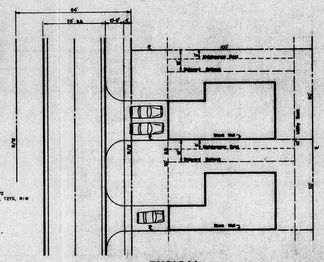
TYPICAL SCALE: 1" = 20'
