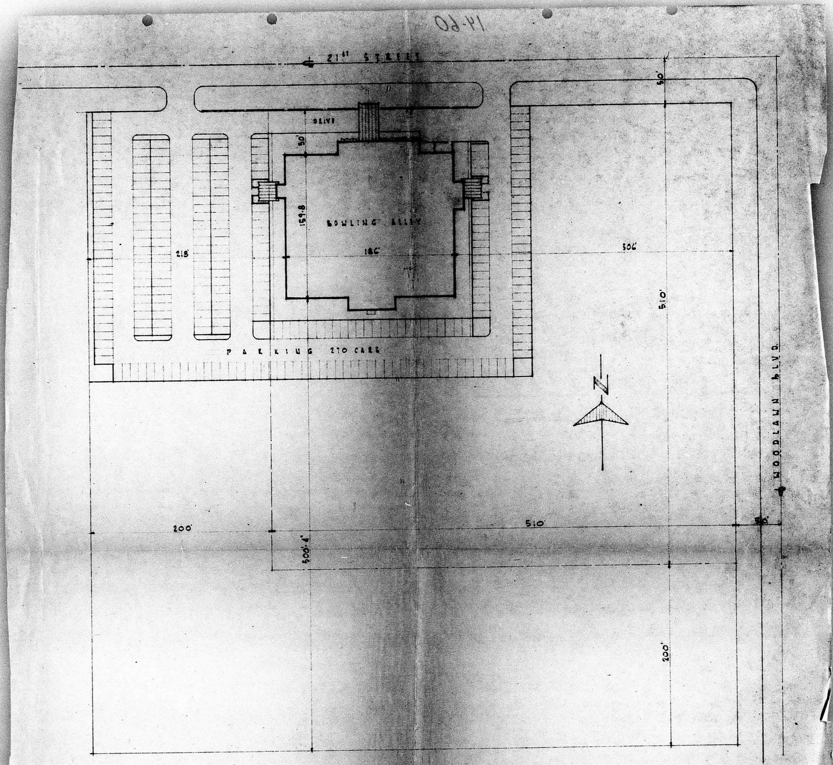
14-60 PLOT PLAN 1" = 50'
