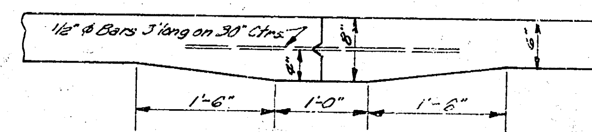
Mastic Joint Detail No Scale
