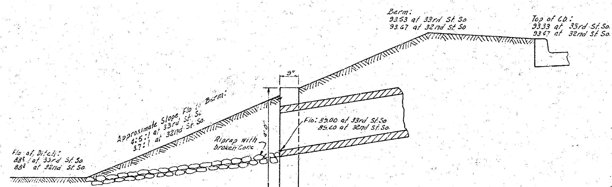
SECTION THRU BANK AT HEADWALL NOT TO SCALE
