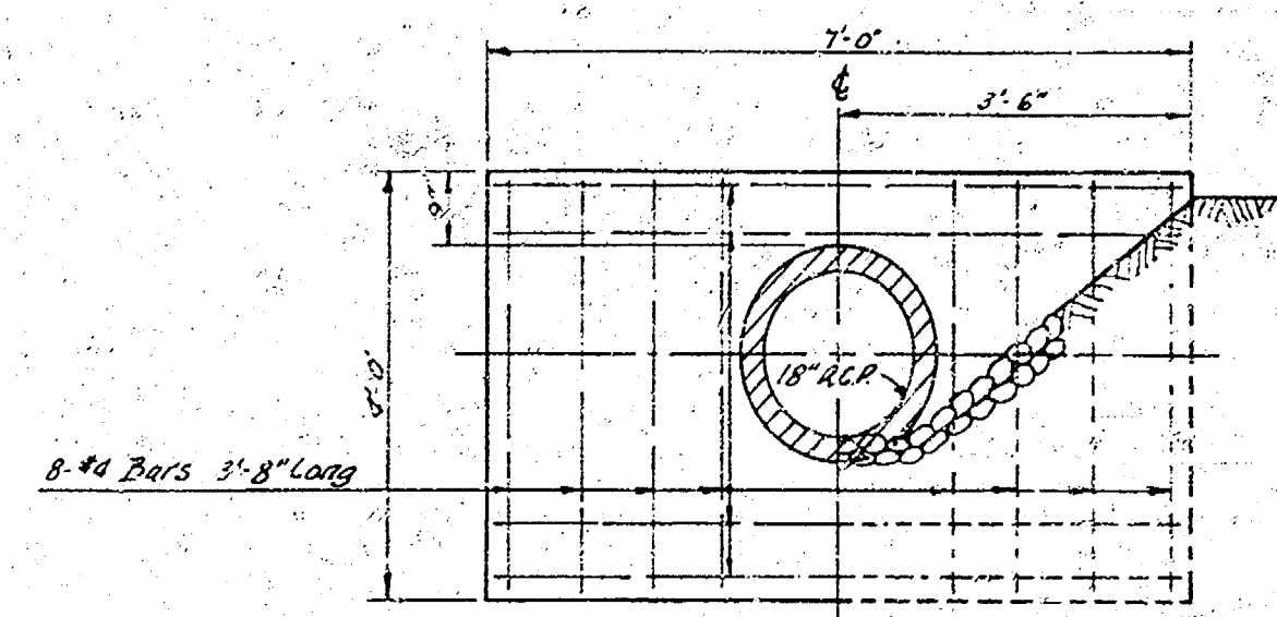
ELEV. OF REINFORCED CONC. HEADWALL NOT TO SCALE SYMMETRICAL ABOUT C
