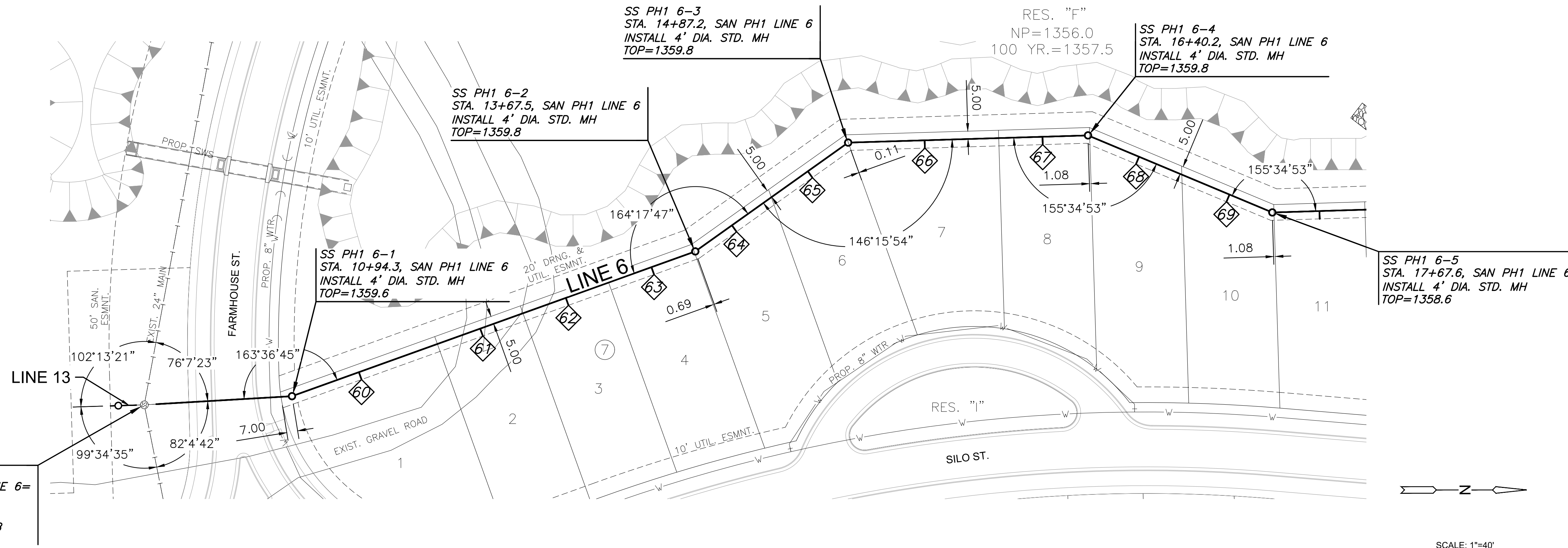
PLAN SAN PH1 LINE 6 PROFILE SAN PH1 LINE 6
