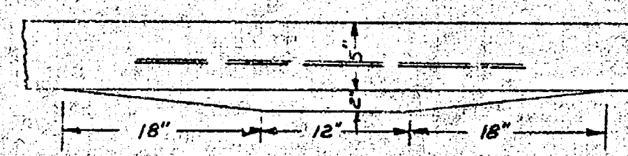
Detail - Keyed Joint No Scale
