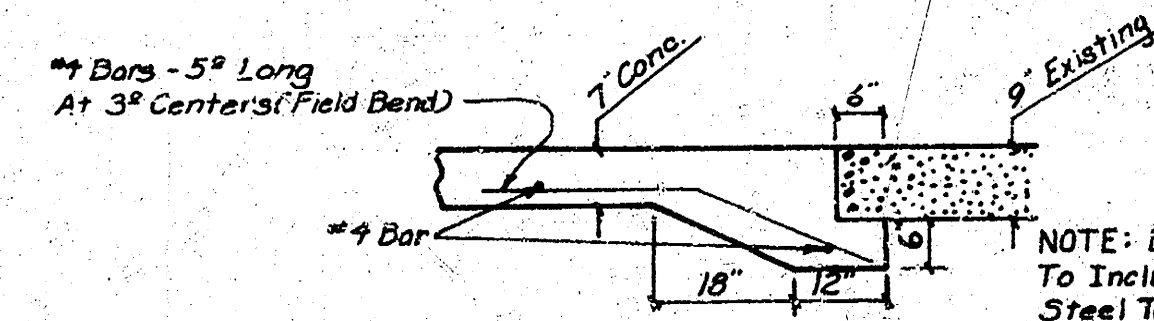
"UNDER-PINNING DETAIL"
