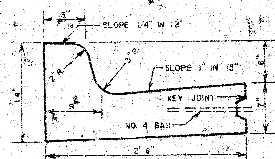
DETAIL OF NON-STANDARD COMBINED CURB & GUTTER
