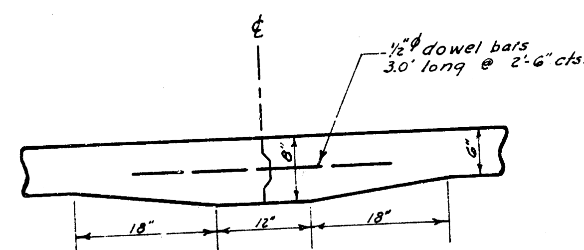
MASTIC JOINT DETAIL
