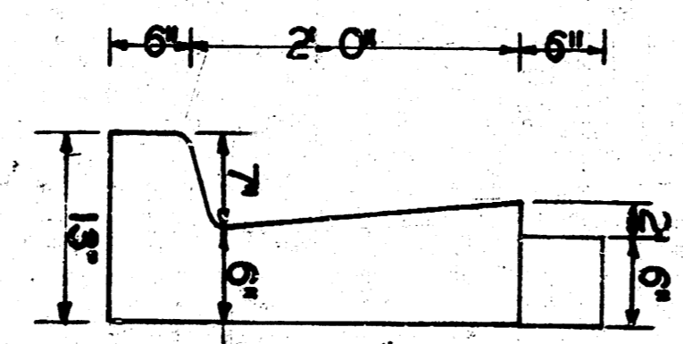
CURB & GUTTER DETAIL
