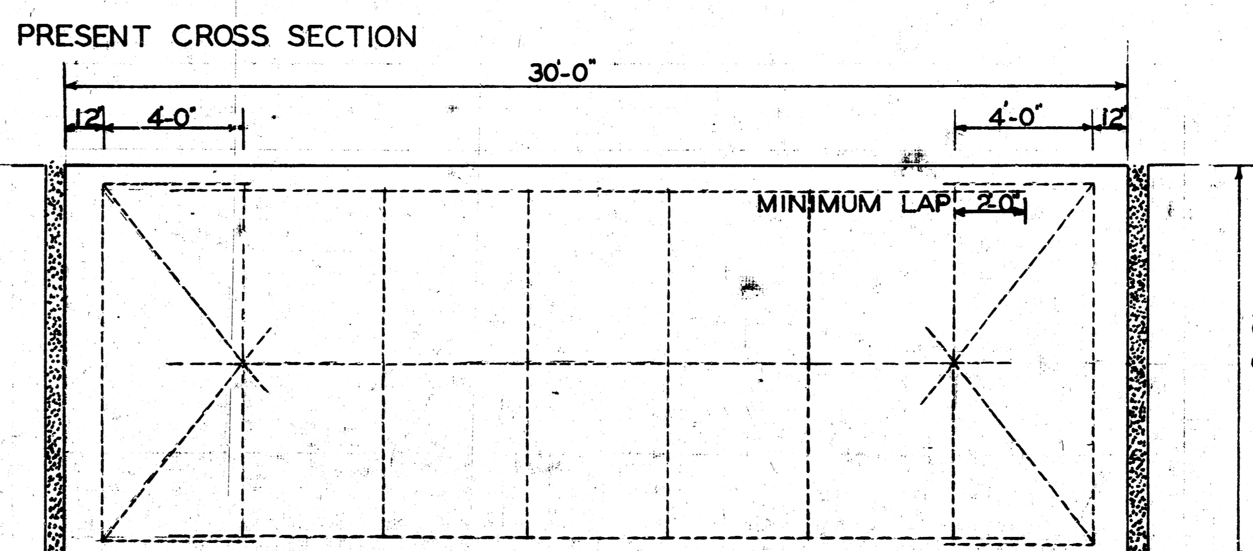
REINFORCING STEEL DETAIL SCALE 3/8"=1'-0"
