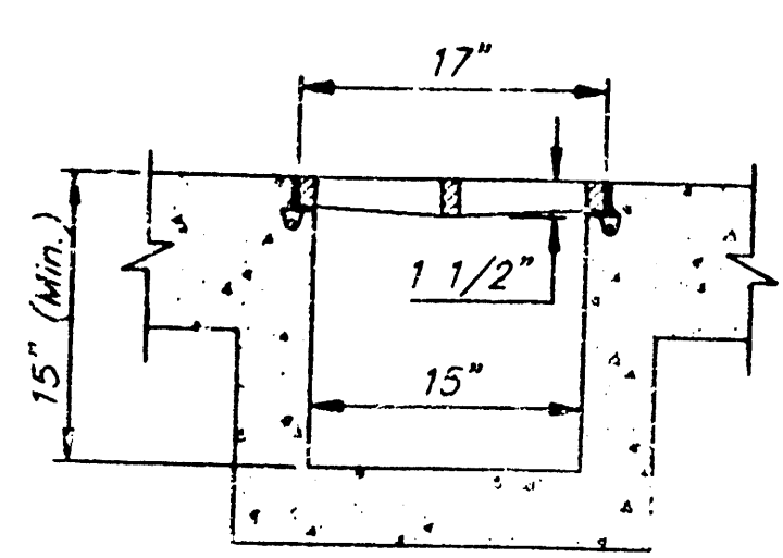
TRENCH DRAIN DETAIL
