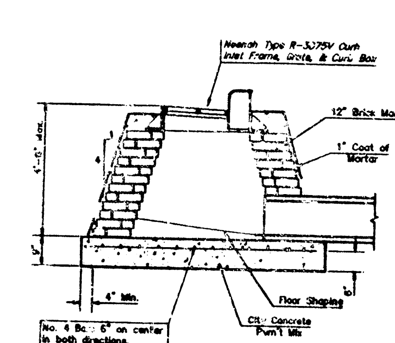
MODIFIED SPECIAL SHALLOW TYPE "B" MANHOLE
