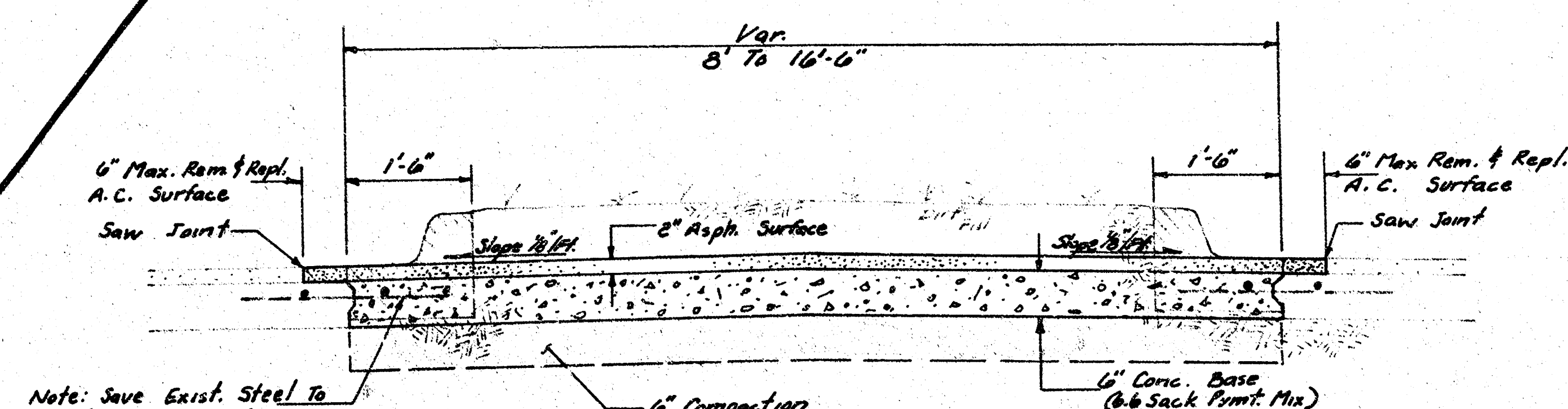
MEDIAL REPLACEMENT DETAIL
