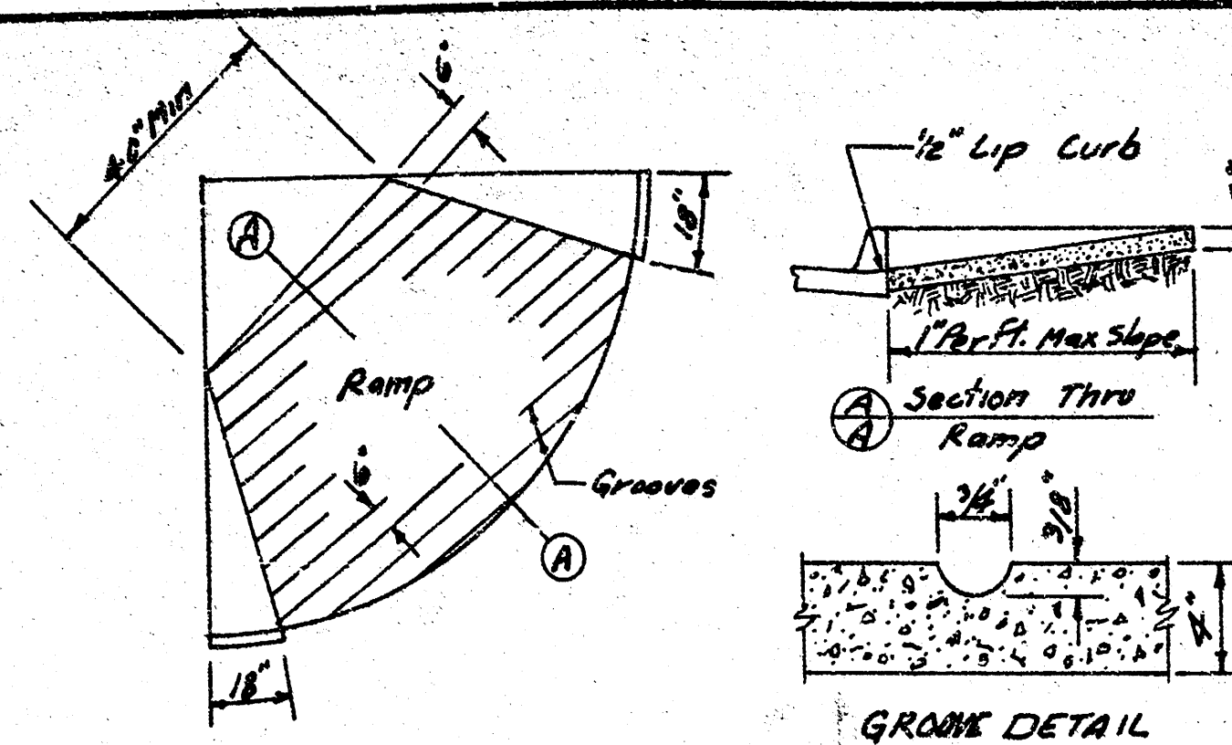
WHEELCHAIR RAMP DETAIL
