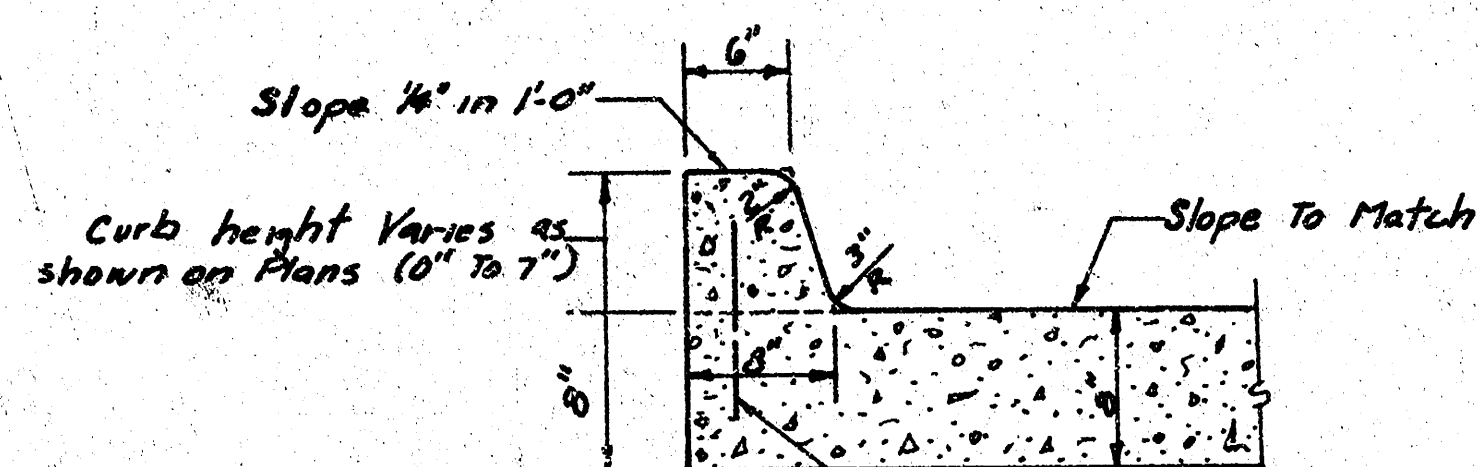
INTEGRAL CURB
