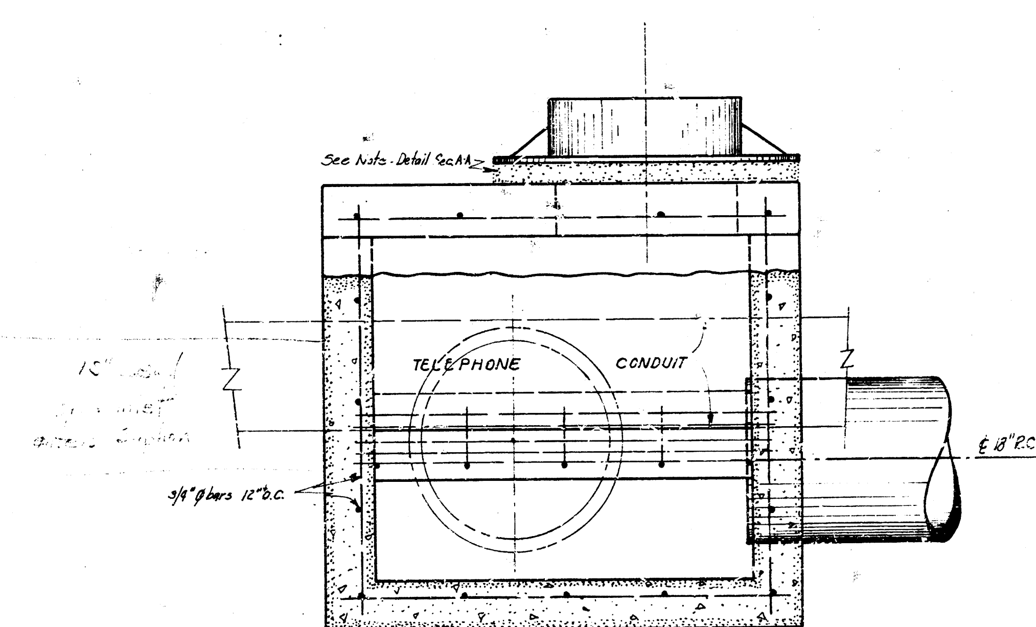
SECTION J-B
