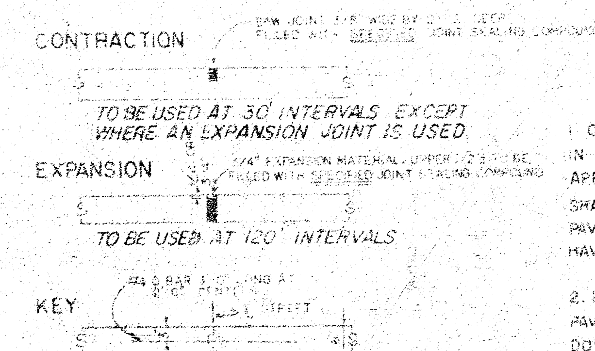
JOINT DETAILS
