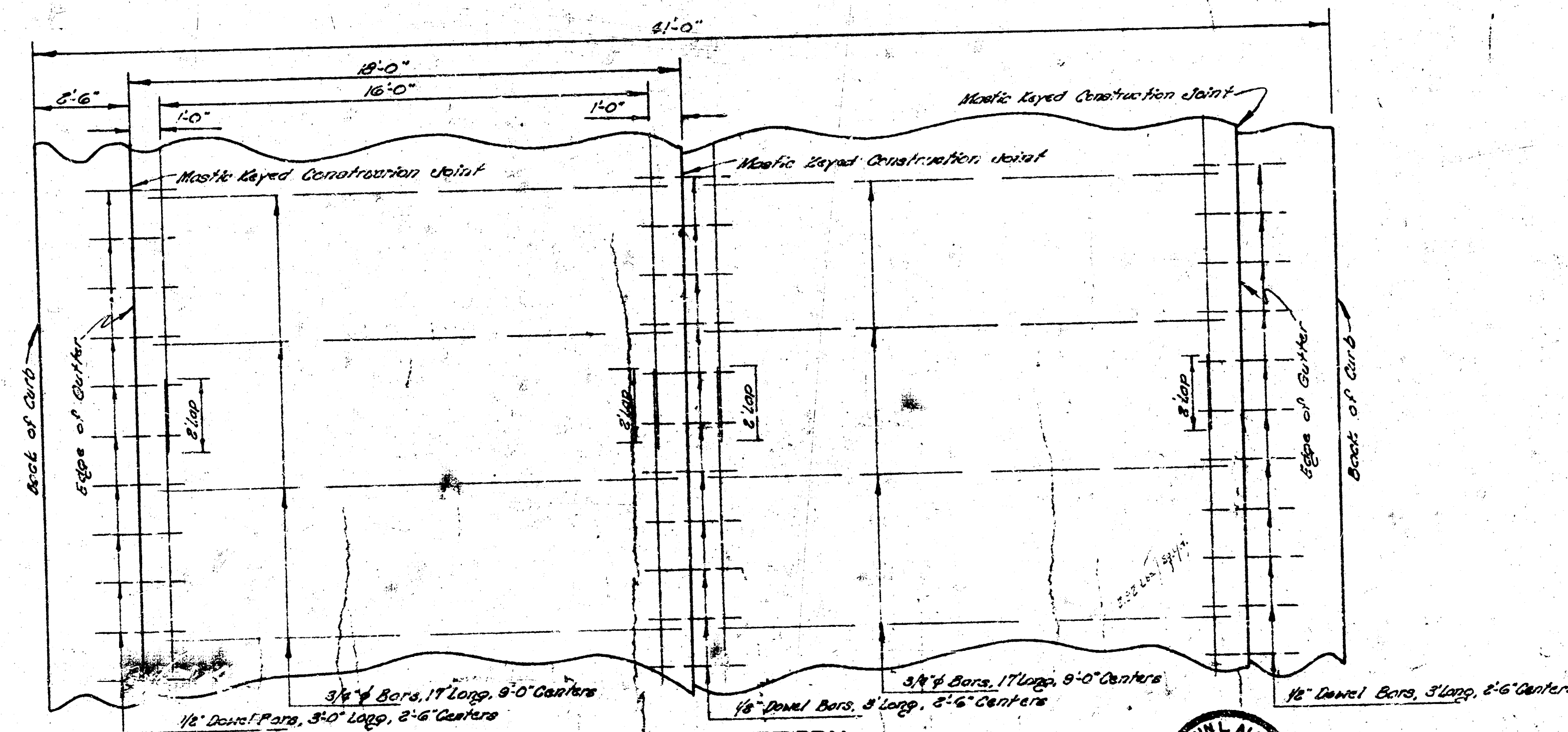
STEEL PATTERN 1/16" 3/4" 0 BARS EXCEPT WHERE NOTED NOT TO SCALE
