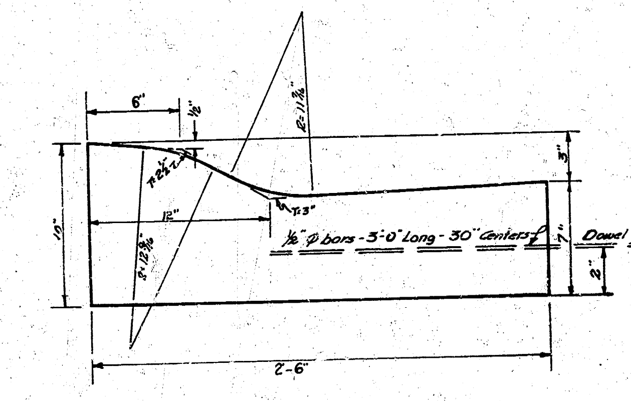
NON-STD. COMB. CURB & GUTTER DETAIL Scale: 2"=1'-0"
