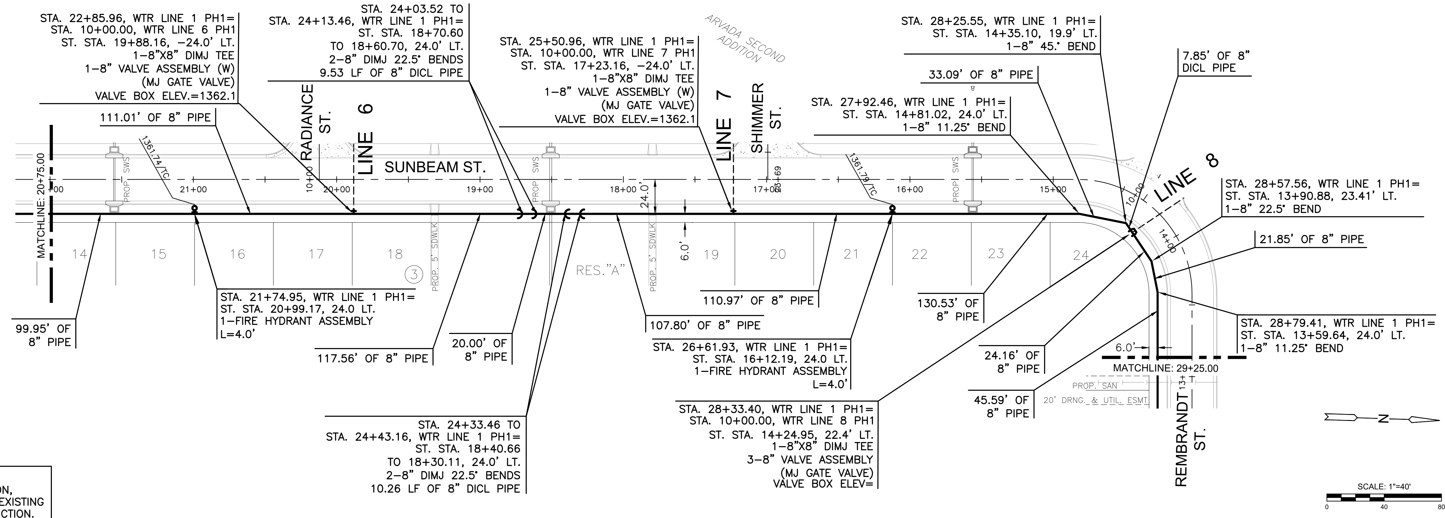
PLAN WTR LINE 1 PH1 CONT. PROFILE WTR LINE 1 PH1 CONT.
