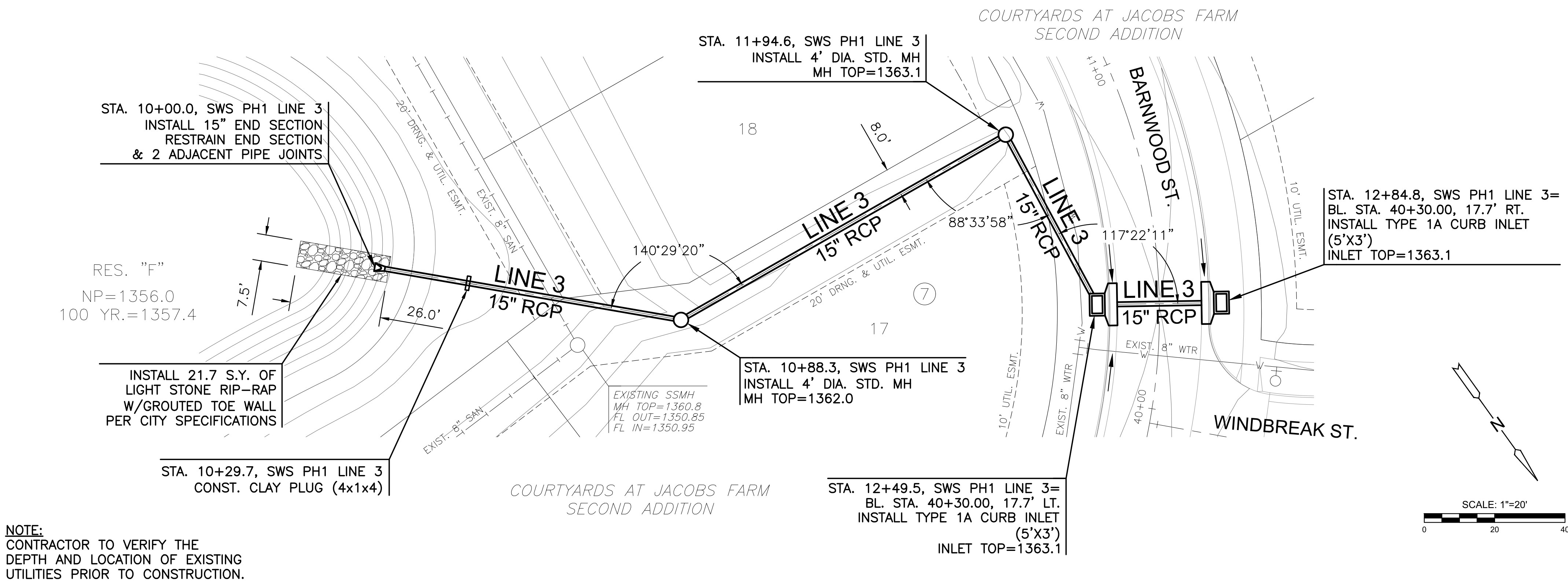
PLAN SWS PH1 LINE 3 PROFILE SWS PH1 LINE 3
