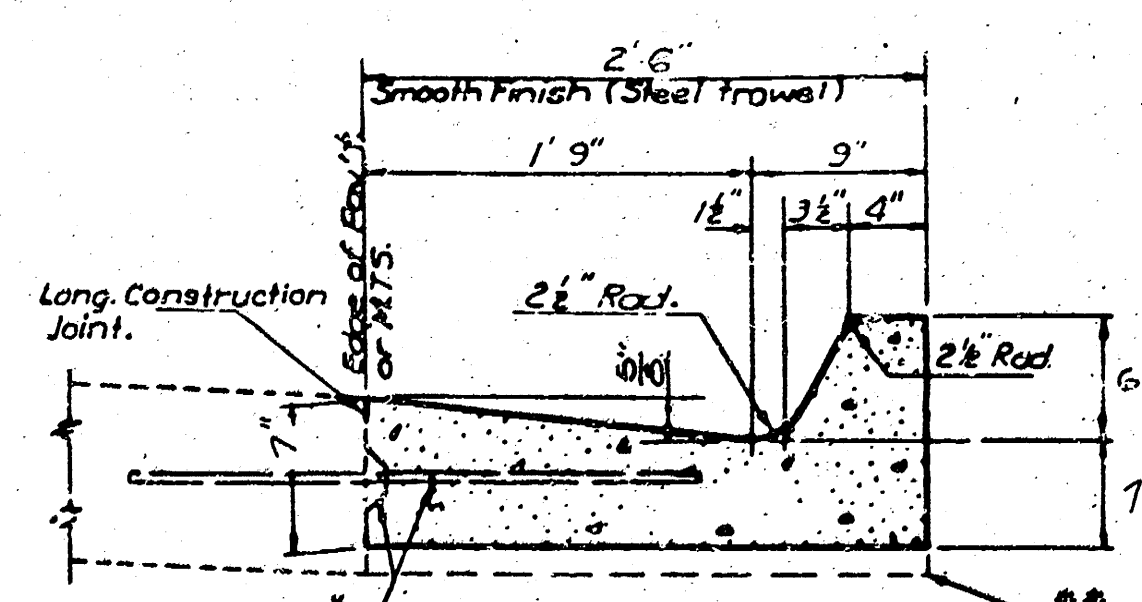
TYPICAL SECTION COMBINED CURB & GUTTER (2'-5\"/>
