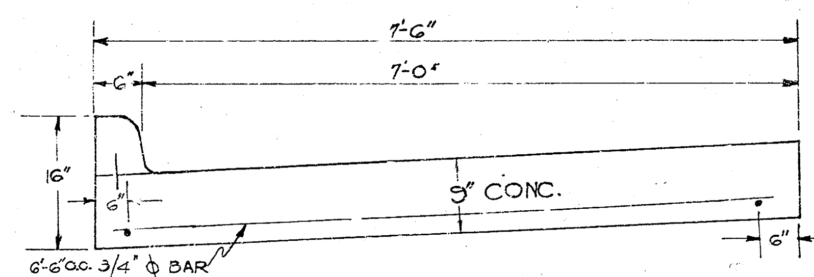
DETAIL OF WIDENING SCALE: 1" = 1'-0"
