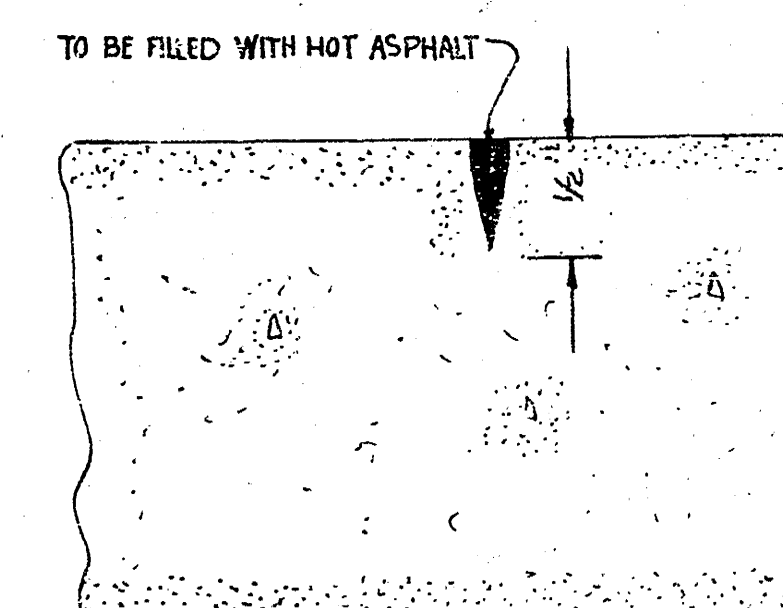
DETAIL OF PLANE OF WEAKNESS NO SCALE
