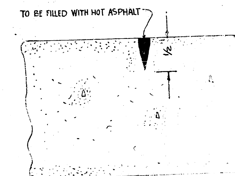
DETAIL OF PLANE OF WEARNESS NO SCALE
