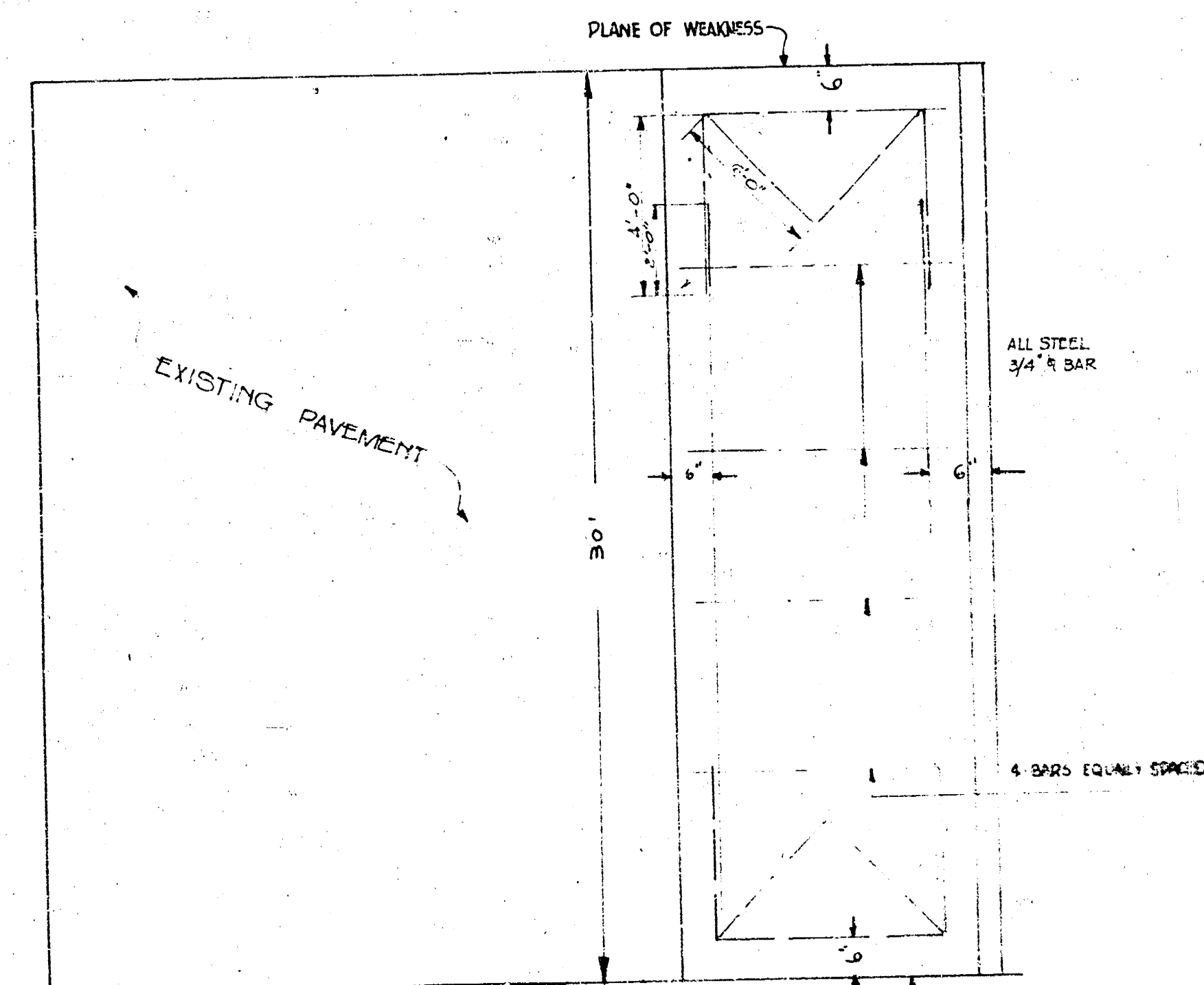
DETAIL OF PLANE OF WEARNESS NO SCALE
