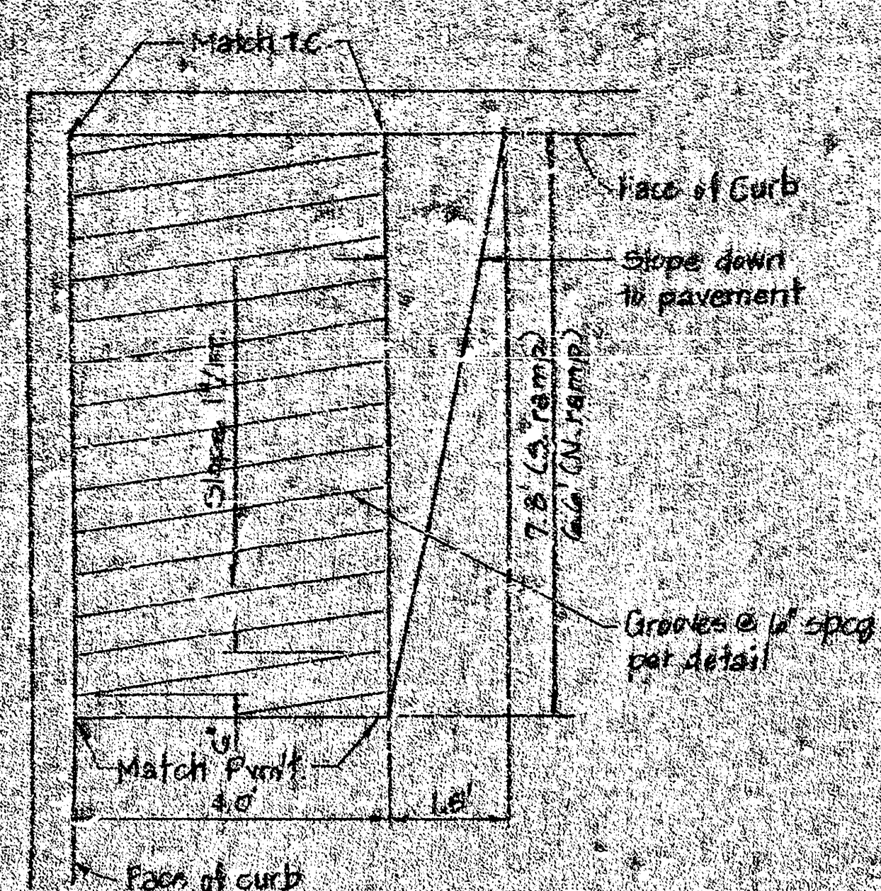
WHEELCHAIR RAMP DETAIL
