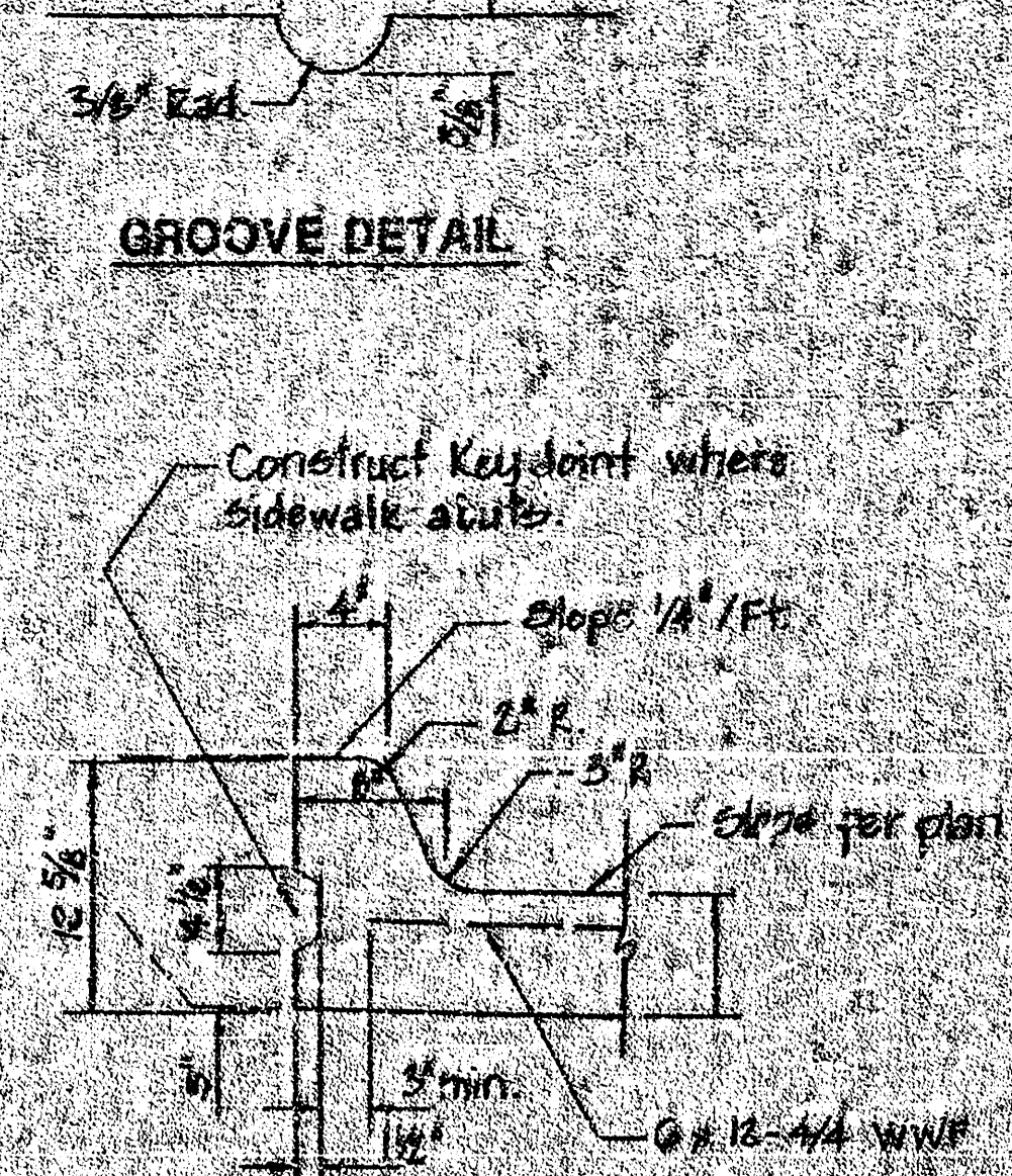
MONOLITHIC CURB DETAIL
