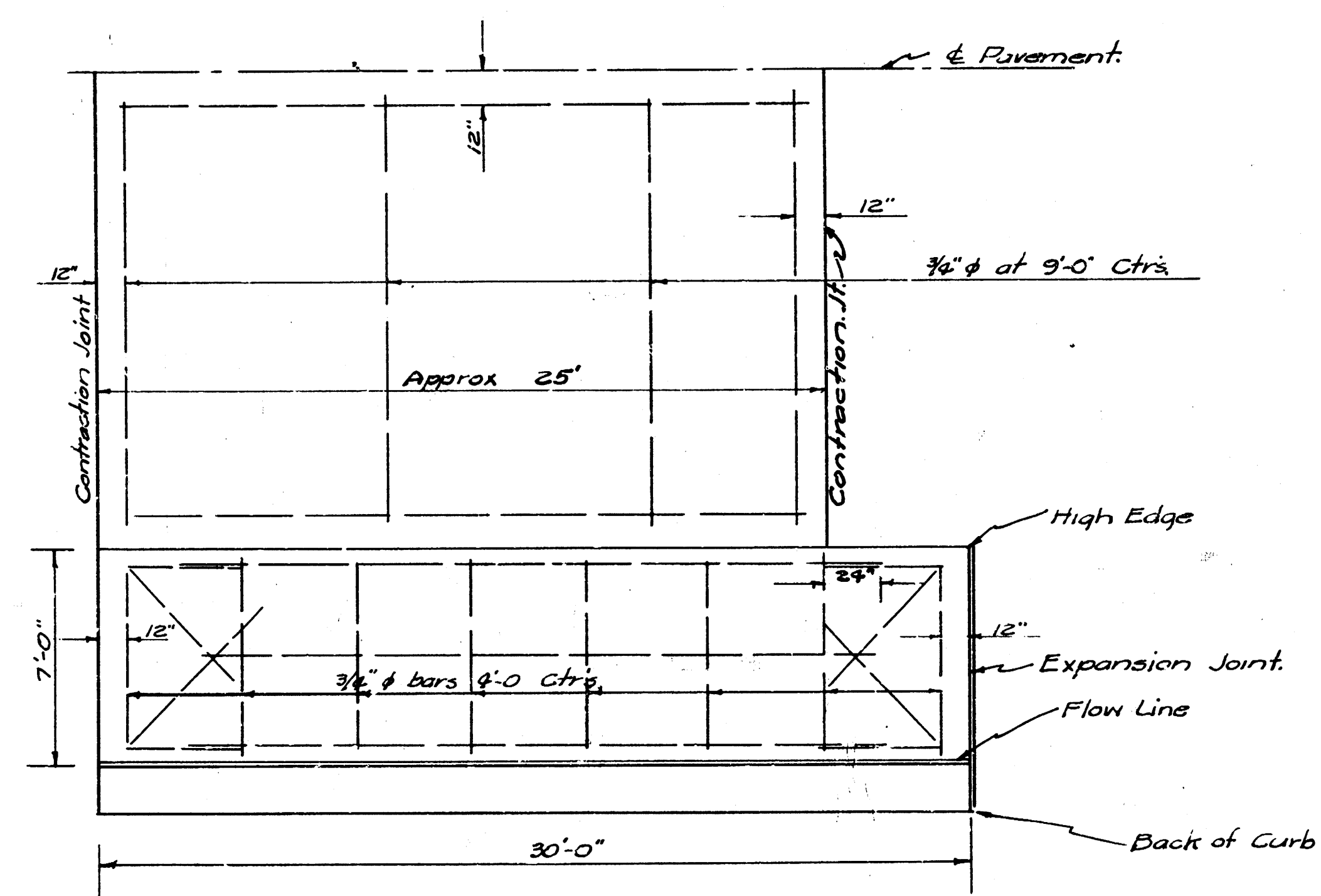
REINFORCING STEEL DETAIL Scale \frac{1}{4}" = 1'
