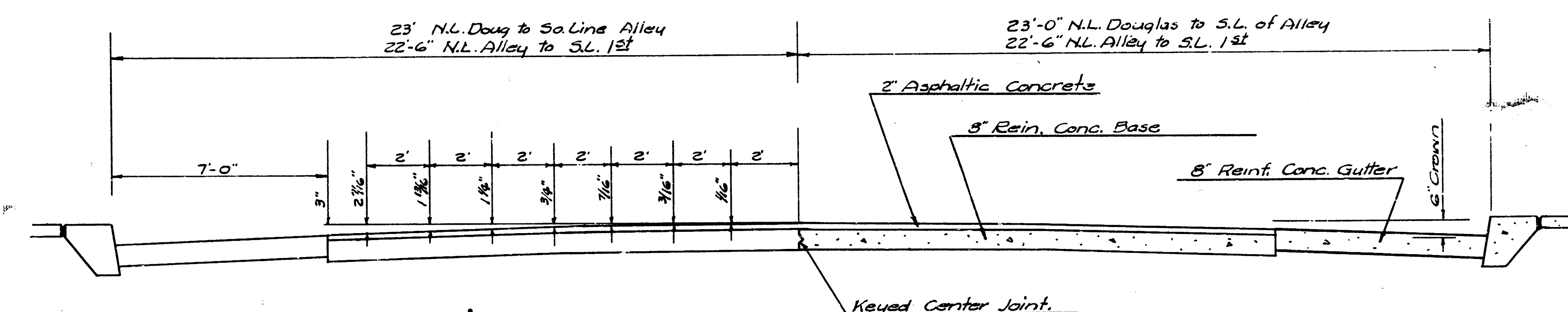
TYPICAL SECTION Scale \frac{3}{8}'' = 1'
