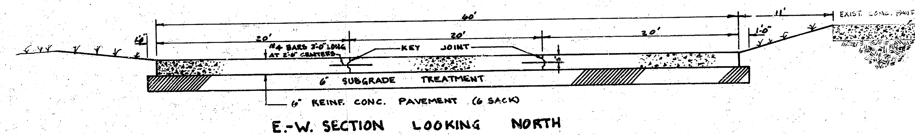
E-W. SECTION LOOKING NORTH
