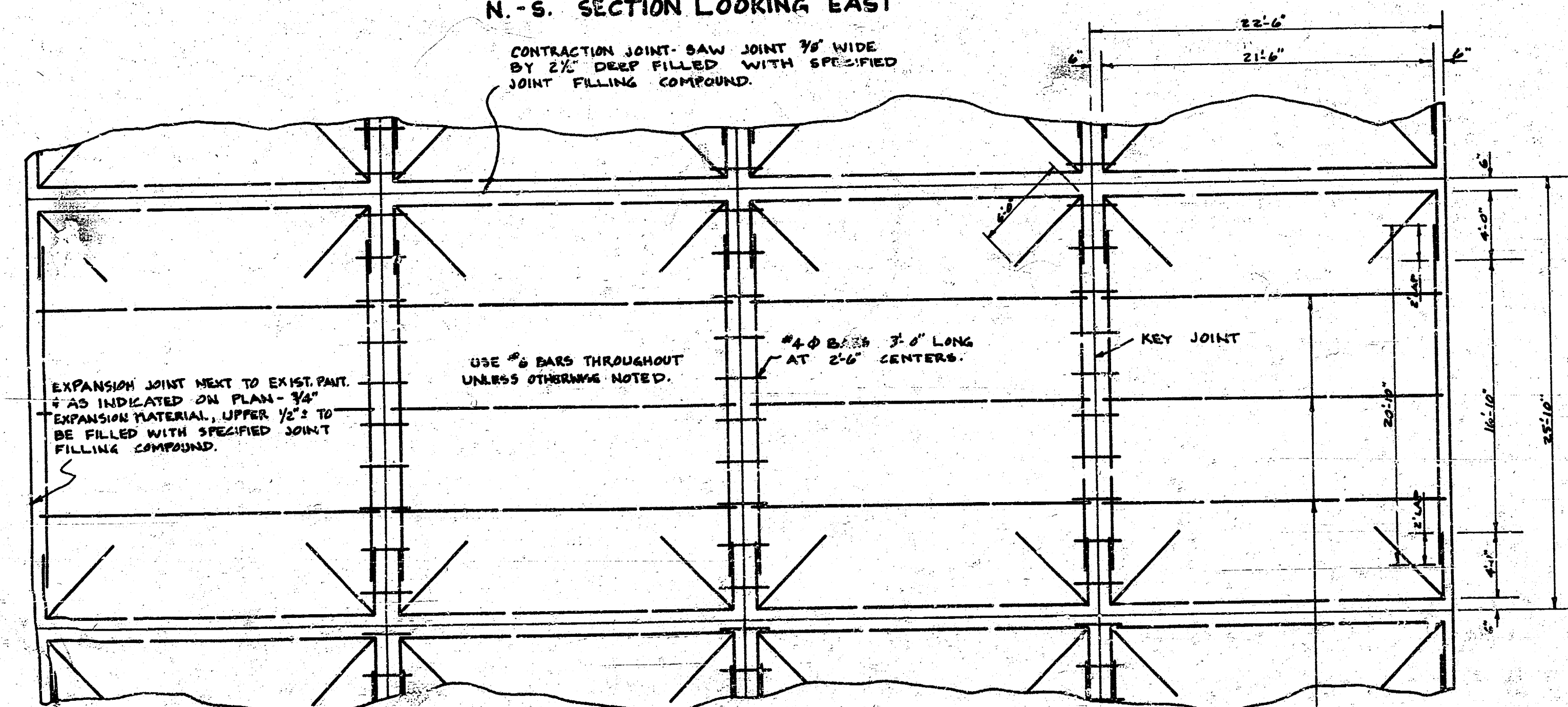
TYPICAL STEEL PATTERN NORTH PARKING LOT
