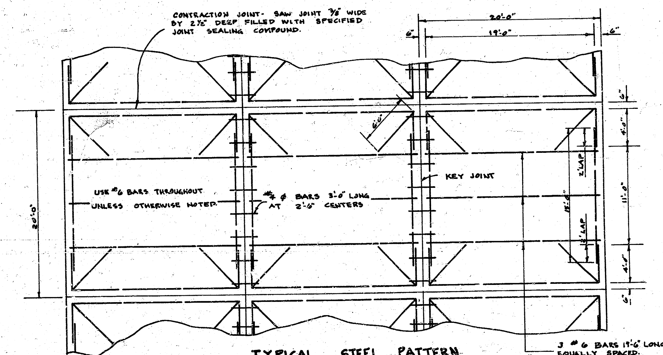
TYPICAL STEEL PATTERN SOUTH PARKING LOT
