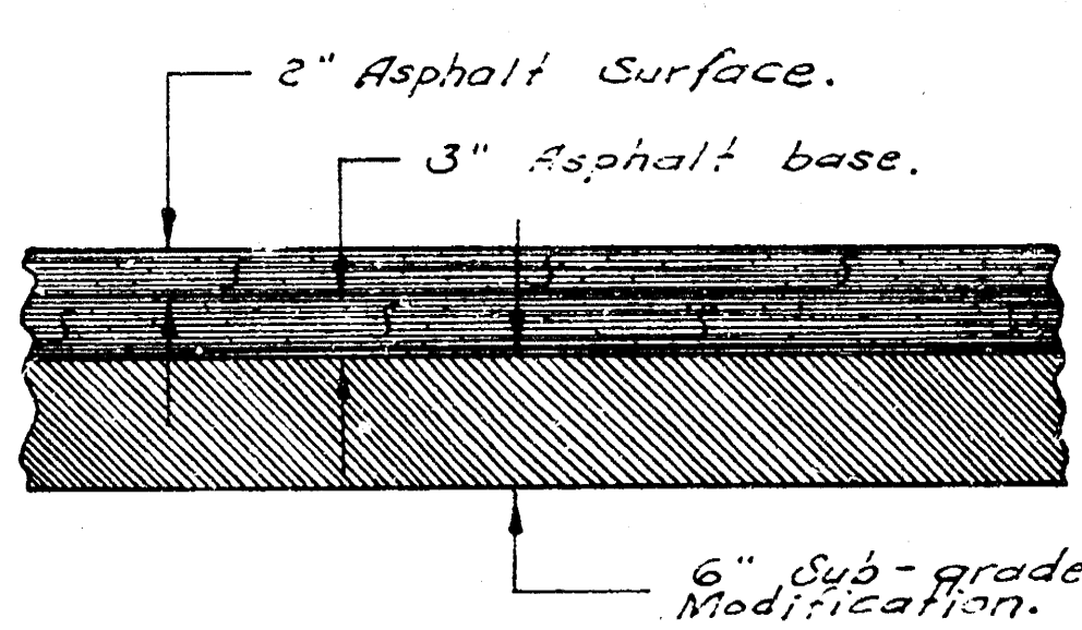
TYPICAL SECTION
