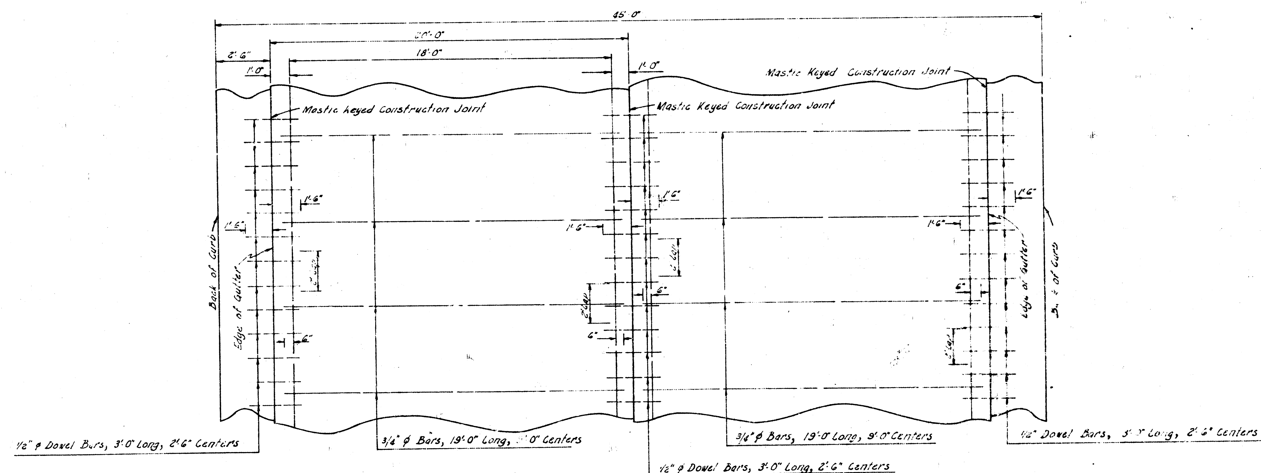
STEEL PATTERN NOT TO SCALE USE 3/4" \phi BARS EXCEPT WHERE NOTED
