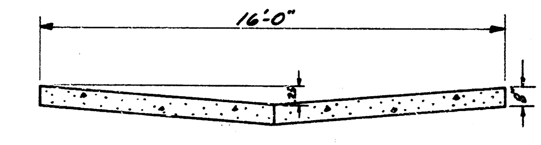
TYPICAL SECTION Sta. 0+50 to Sta. 4+02.8 No Scale
