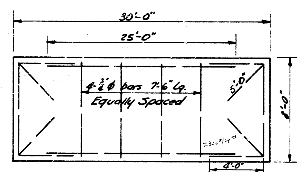
STEEL PATTERN No Scale
