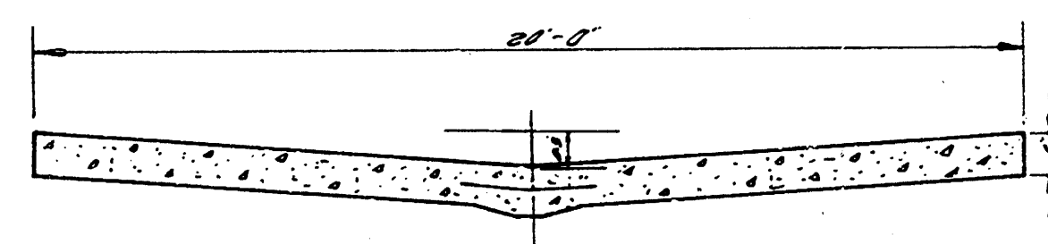
TYPICAL SECTION (EXCEPTION AT WARPED SECTION) NO SCALE
