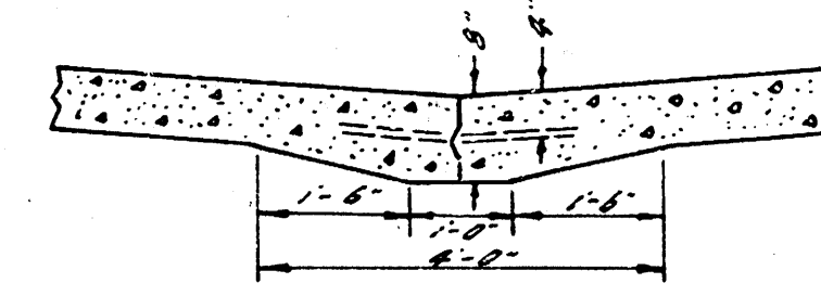
DETAIL OF DYNASTIC KEY JOINT NO SCALE
