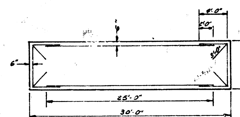
STEEL PATTERN NOT TO SCALE
