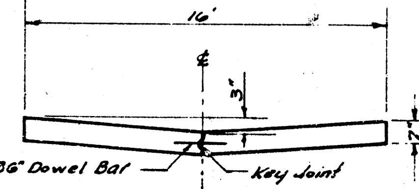
TYPICAL SECTION No Scale:
