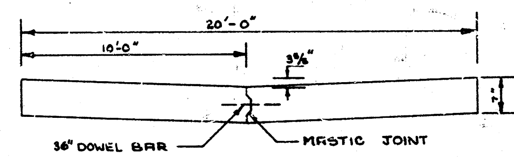
TYPICAL SECTION NO SCALE
