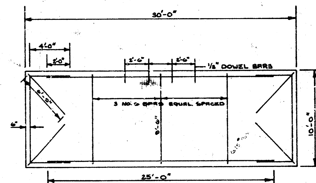
STEEL PATTERN NO SCALE
