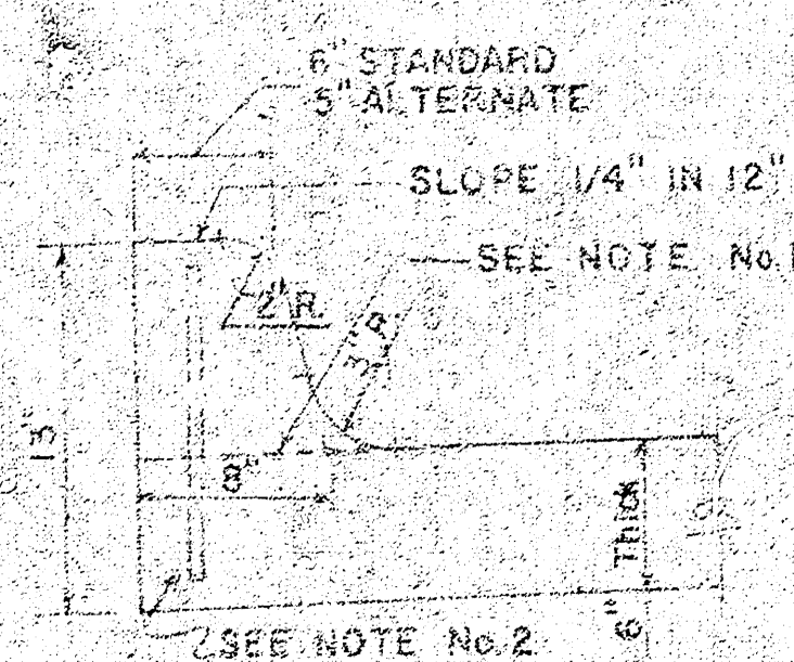
INTEGRAL CURB
