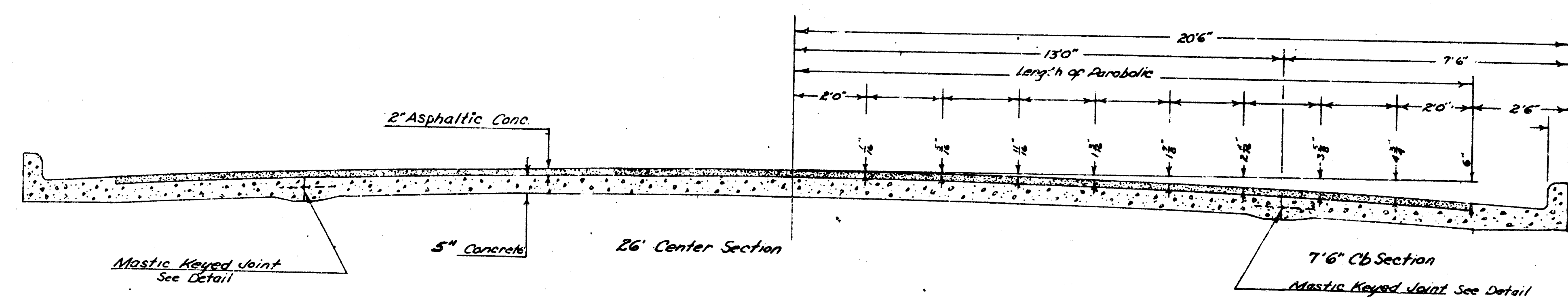
TYPICAL SECTION
