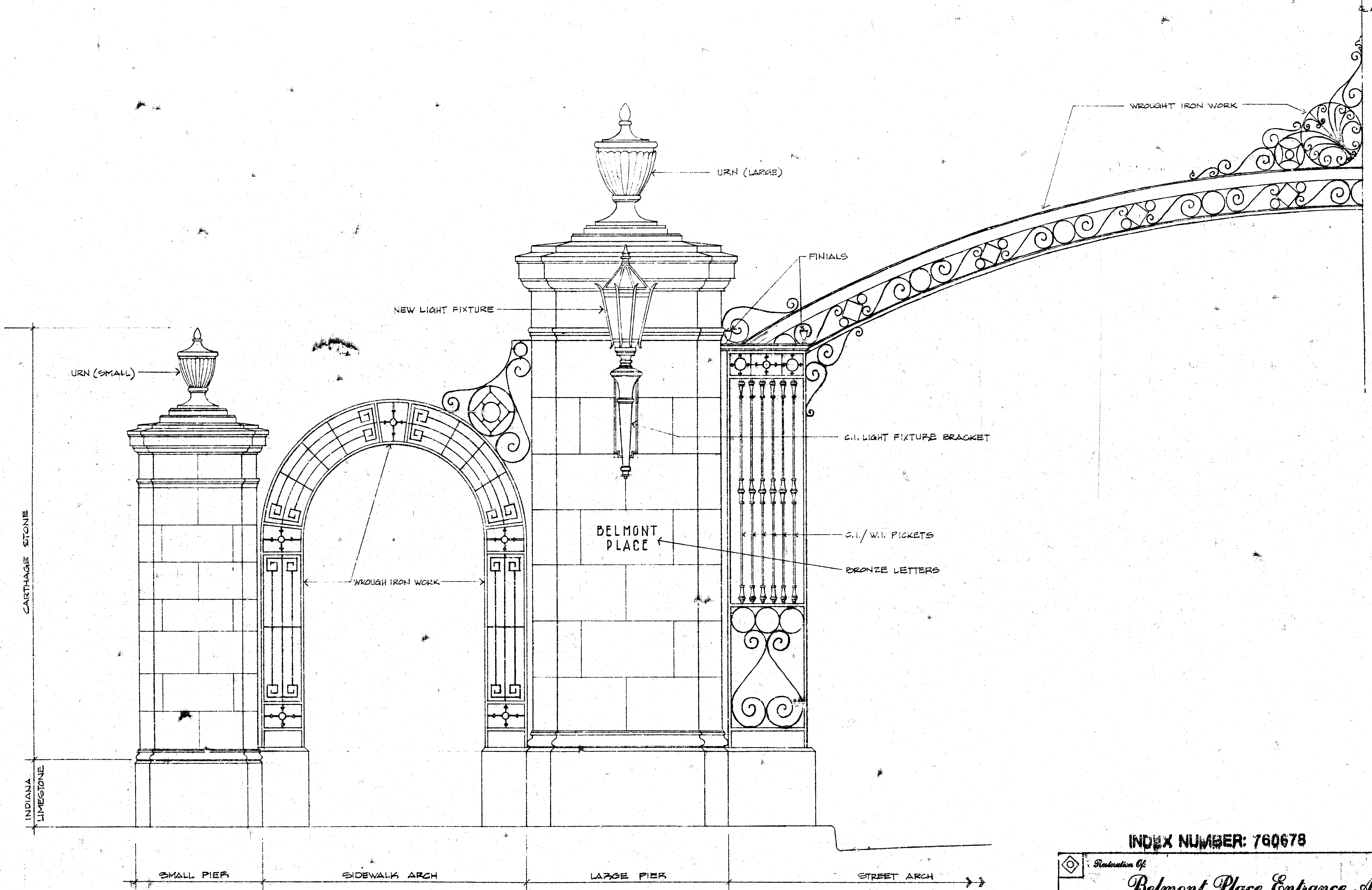
HALF ELEVATION OF STREET ENTRANCE SCALE: 3/4" = 1'-0"
