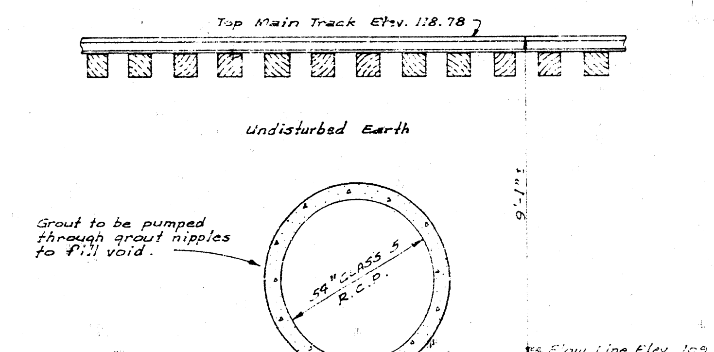
TYPICAL SECTION SANTA FE R.R. CROSSING STA. 201291 TO 311311 Note: Pipe to be installed by jacking method
