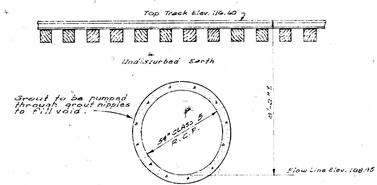
TYPICAL SECTION FRISCO R.R. CROSSING STA. 91891 TO 101191 Note: Pipe to be installed by jacking method
