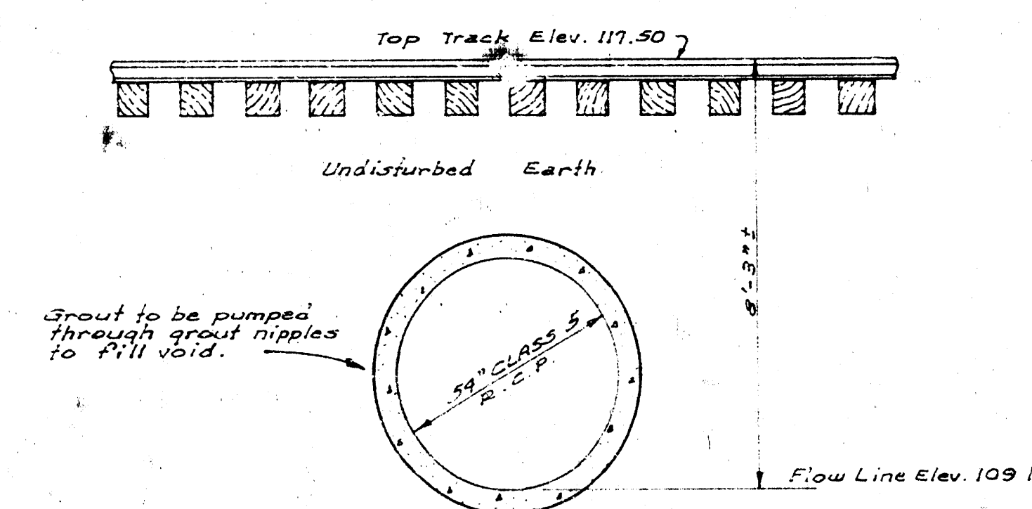
TYPICAL SECTION ROCK ISLAND R.R. CROSSING STA. 151991 TO 161291 Note: Pipe to be installed by jacking method
