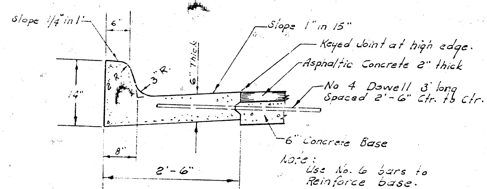
STANDARD SECTION OF COMBINED CURB & GUTTER
