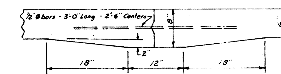
DETAIL of MASTIC KEYED JOINT No Scale
