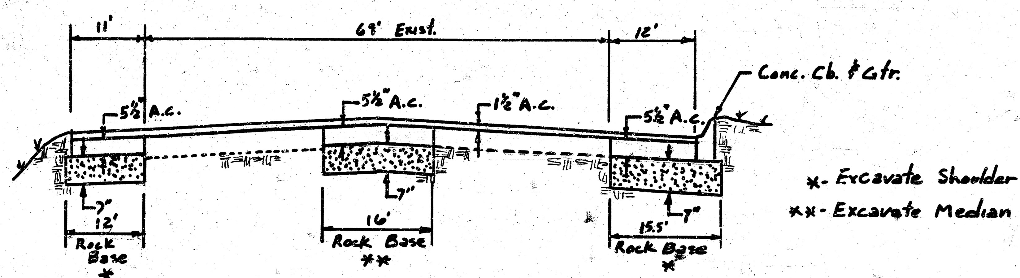
SECTION B-B
