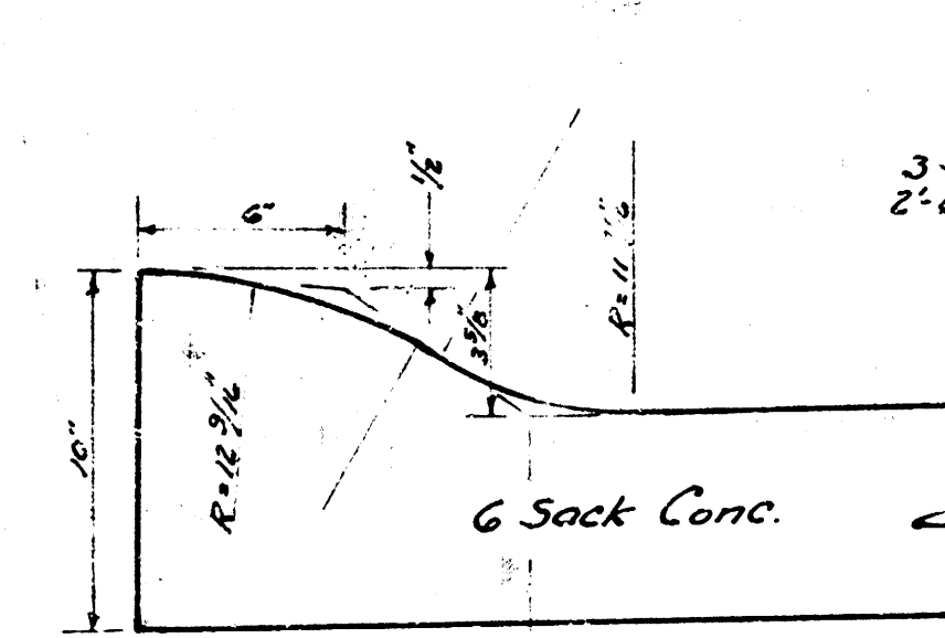
ROLL CURB DETAIL No Scale
