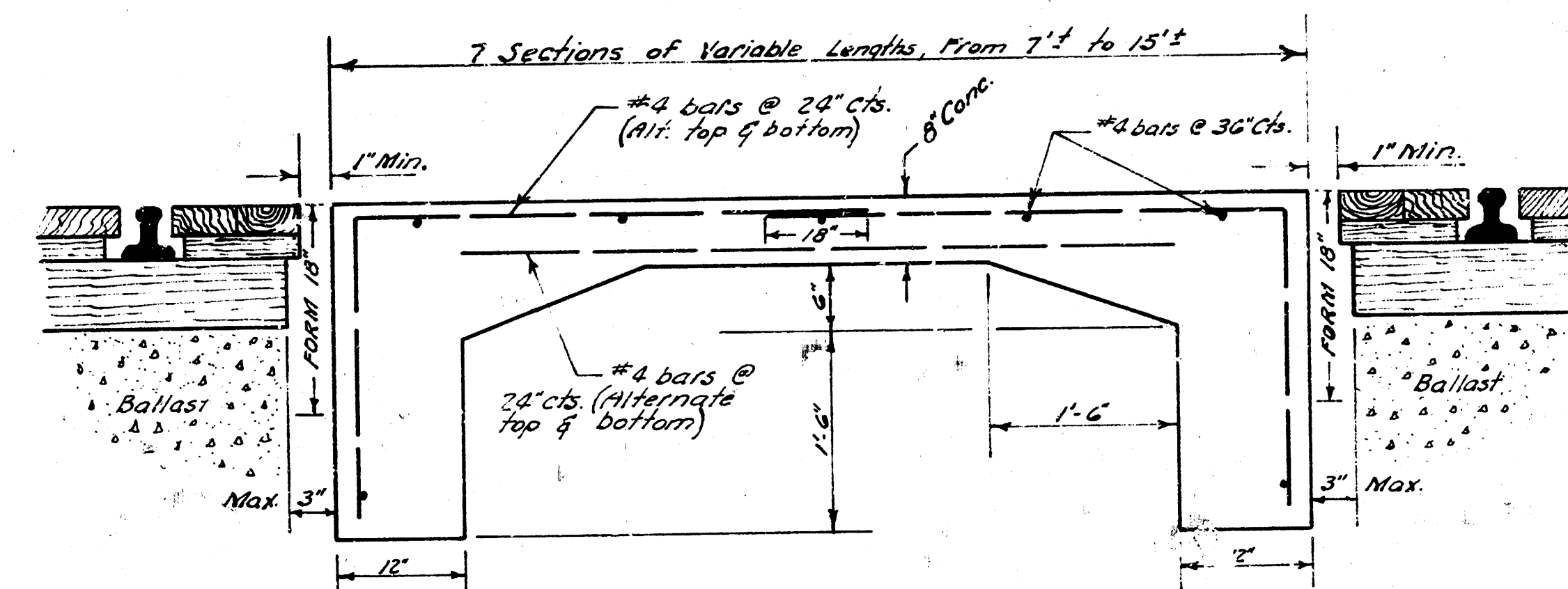
CONC. PAVEMENT & HEADER DETAIL BETWEEN TRACKS No Scale
