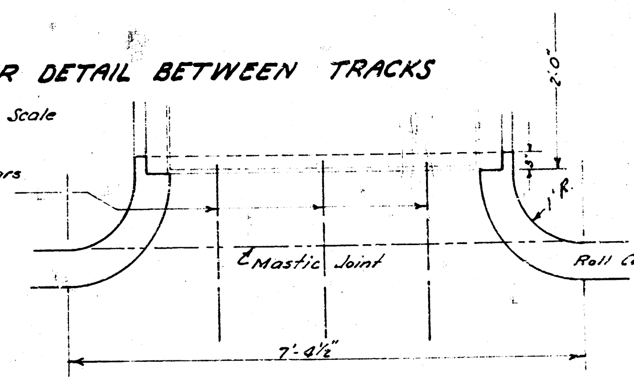
PLAN VIEW OF SETBACK FOR 2'x5' INLET No Scale
