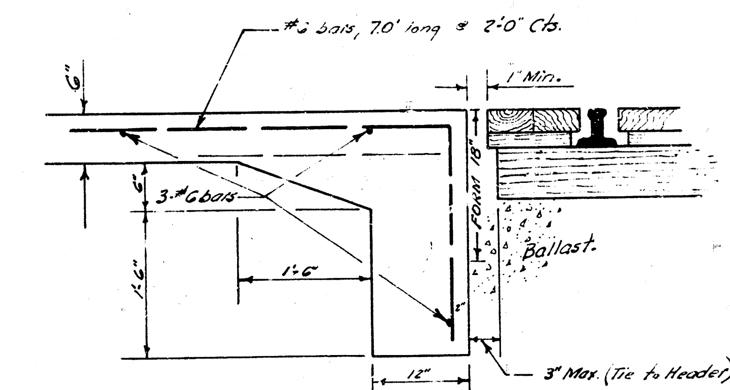
CONC. HEADER DETAIL FOR R.R. CROSSINGS No Scale
